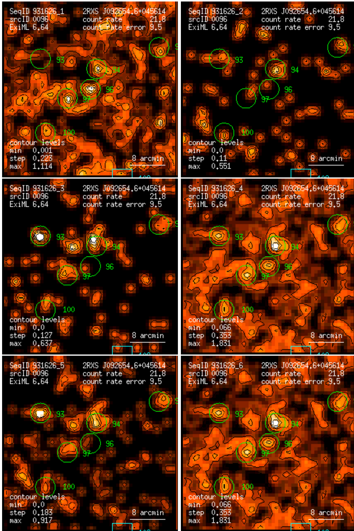
Figure 96: RASS 931626: detection 0096: band rate images, Gaussian filter: (1) PSPC channels 11 – 41, (2) 52 – 90, (3) 91 – 201, (4) 11 – 235, (5) 52 – 201, (6) 11 – 201. Broad band rates in counts/ks. Band rate contour levels in counts/ks/arcmin 2 .
