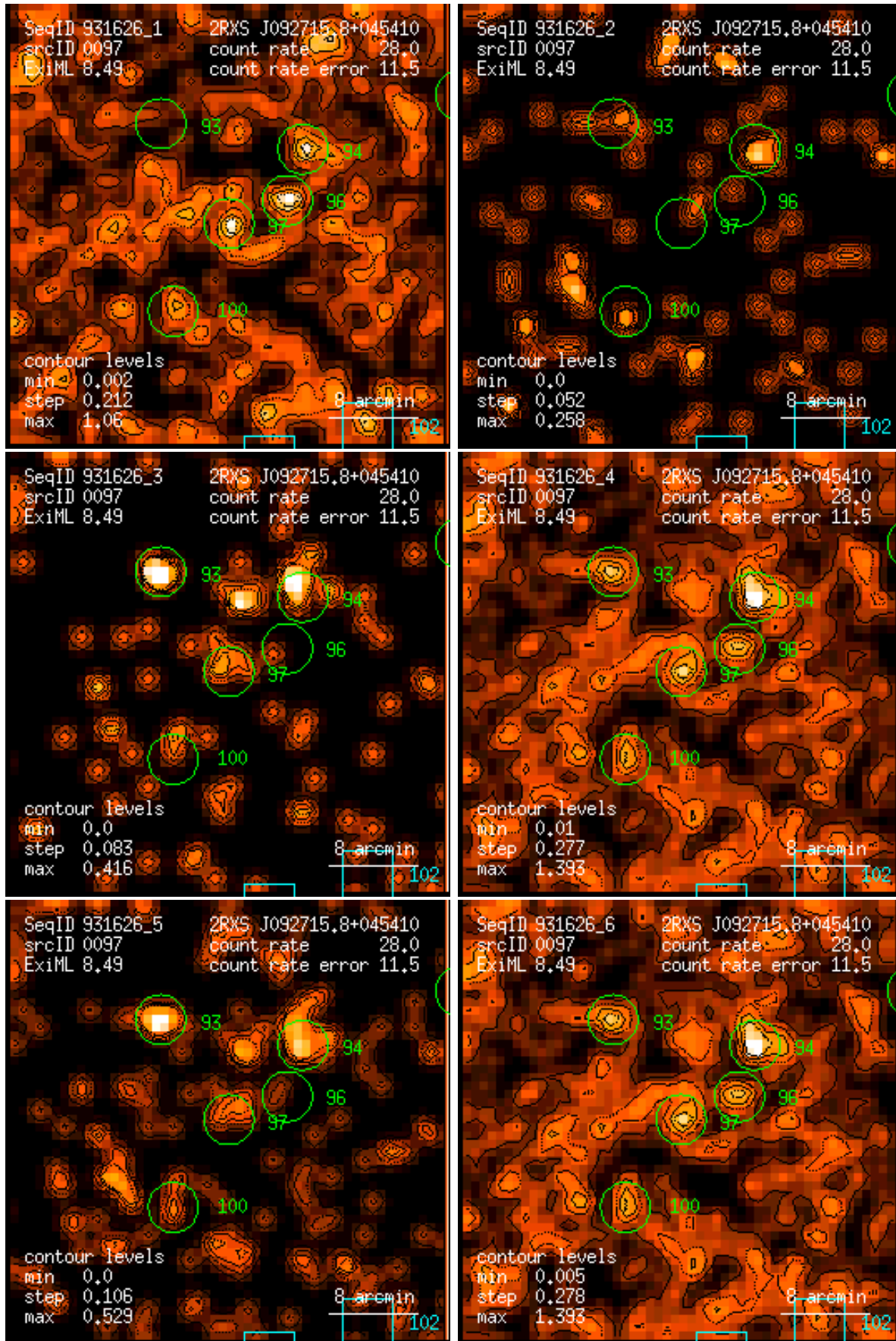
Figure 97: RASS 931626: detection 0097: band rate images, Gaussian filter: (1) PSPC channels 11 – 41, (2) 52 – 90, (3) 91 – 201, (4) 11 – 235, (5) 52 – 201, (6) 11 – 201. Broad band rates in counts/ks. Band rate contour levels in counts/ks/arcmin 2 .
