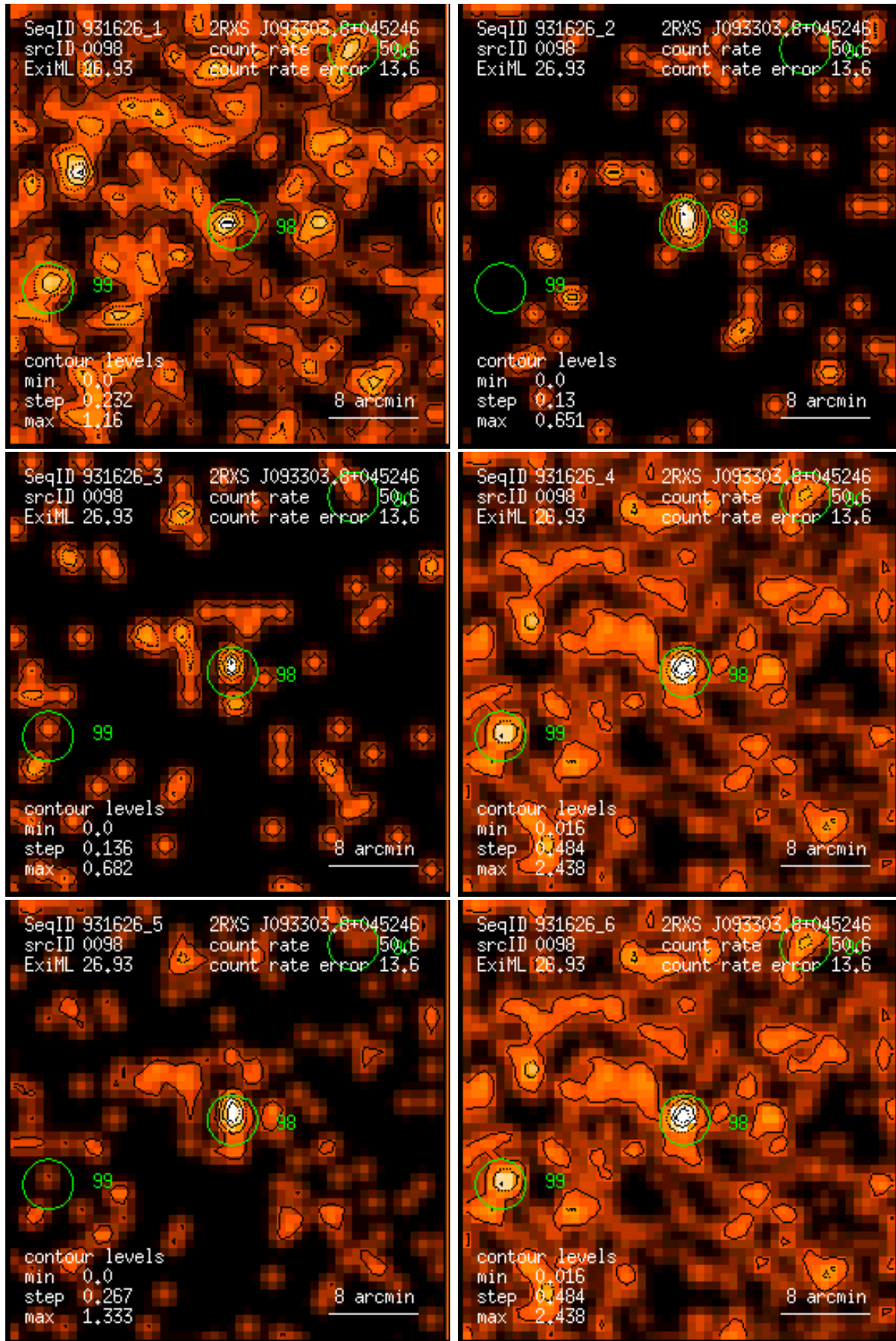
Figure 98: RASS 931626: detection 0098: band rate images, Gaussian filter: (1) PSPC channels 11 – 41, (2) 52 – 90, (3) 91 – 201, (4) 11 – 235, (5) 52 – 201, (6) 11 – 201. Broad band rates in counts/ks. Band rate contour levels in counts/ks/arcmin 2 .
