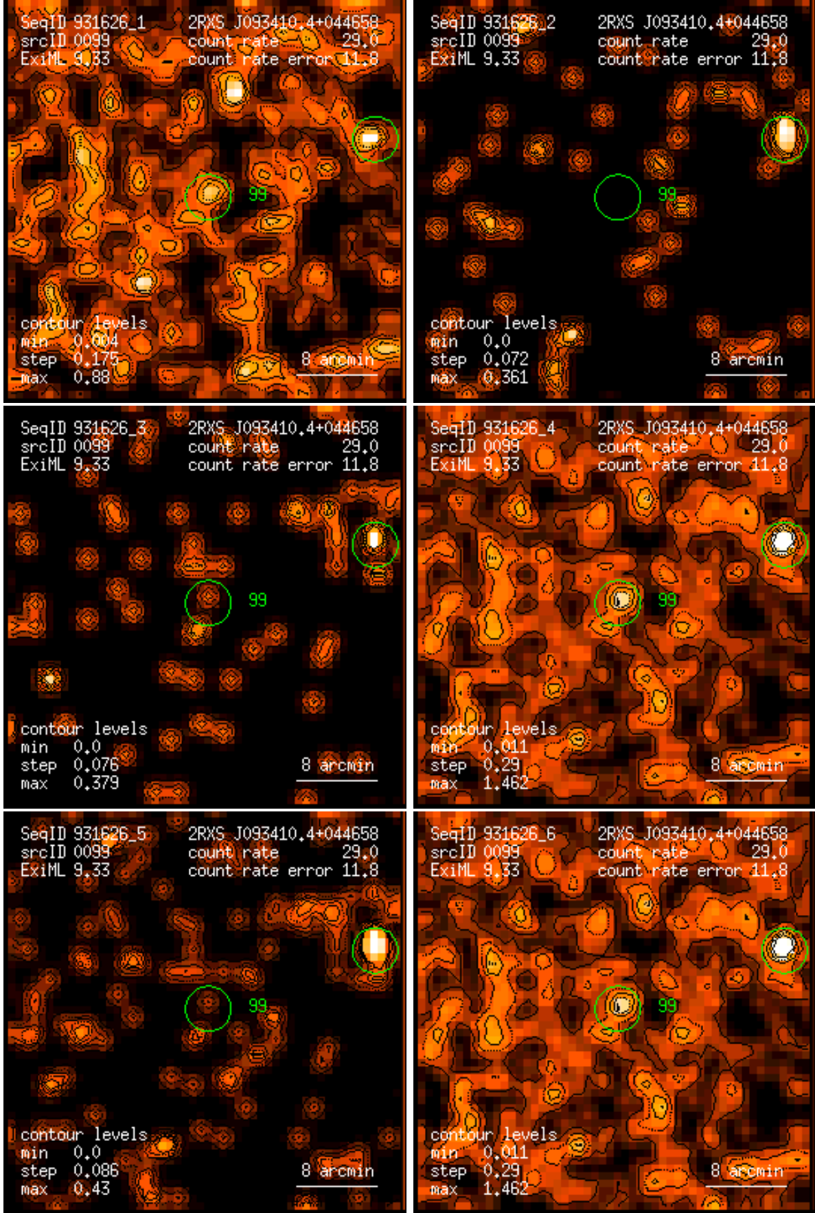
Figure 99: RASS 931626: detection 0099: band rate images, Gaussian filter: (1) PSPC channels 11 – 41, (2) 52 – 90, (3) 91 – 201, (4) 11 – 235, (5) 52 – 201, (6) 11 – 201. Broad band rates in counts/ks. Band rate contour levels in counts/ks/arcmin 2 .
