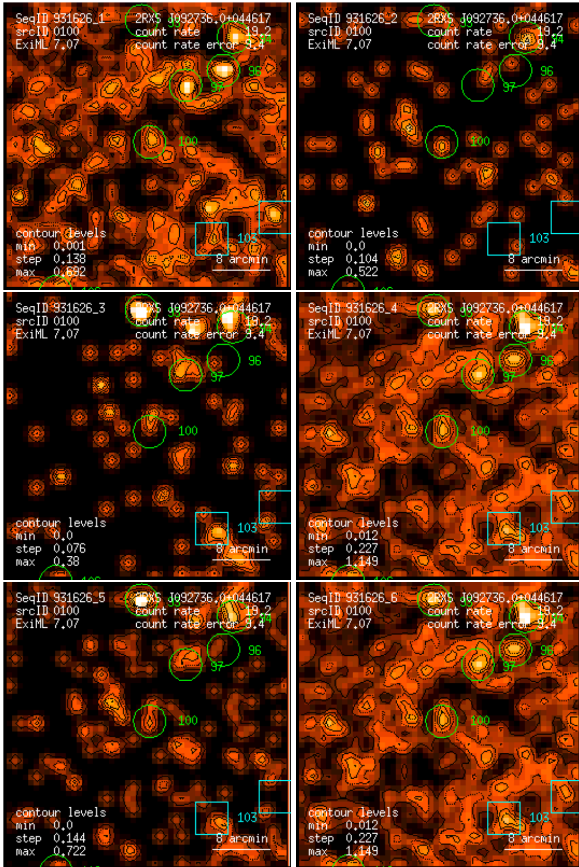
Figure 100: RASS 931626: detection 0100: band rate images, Gaussian filter: (1) PSPC channels 11 – 41, (2) 52 – 90, (3) 91 – 201, (4) 11 – 235, (5) 52 – 201, (6) 11 – 201. Broad band rates in counts/ks. Band rate contour levels in counts/ks/arcmin 2 .
