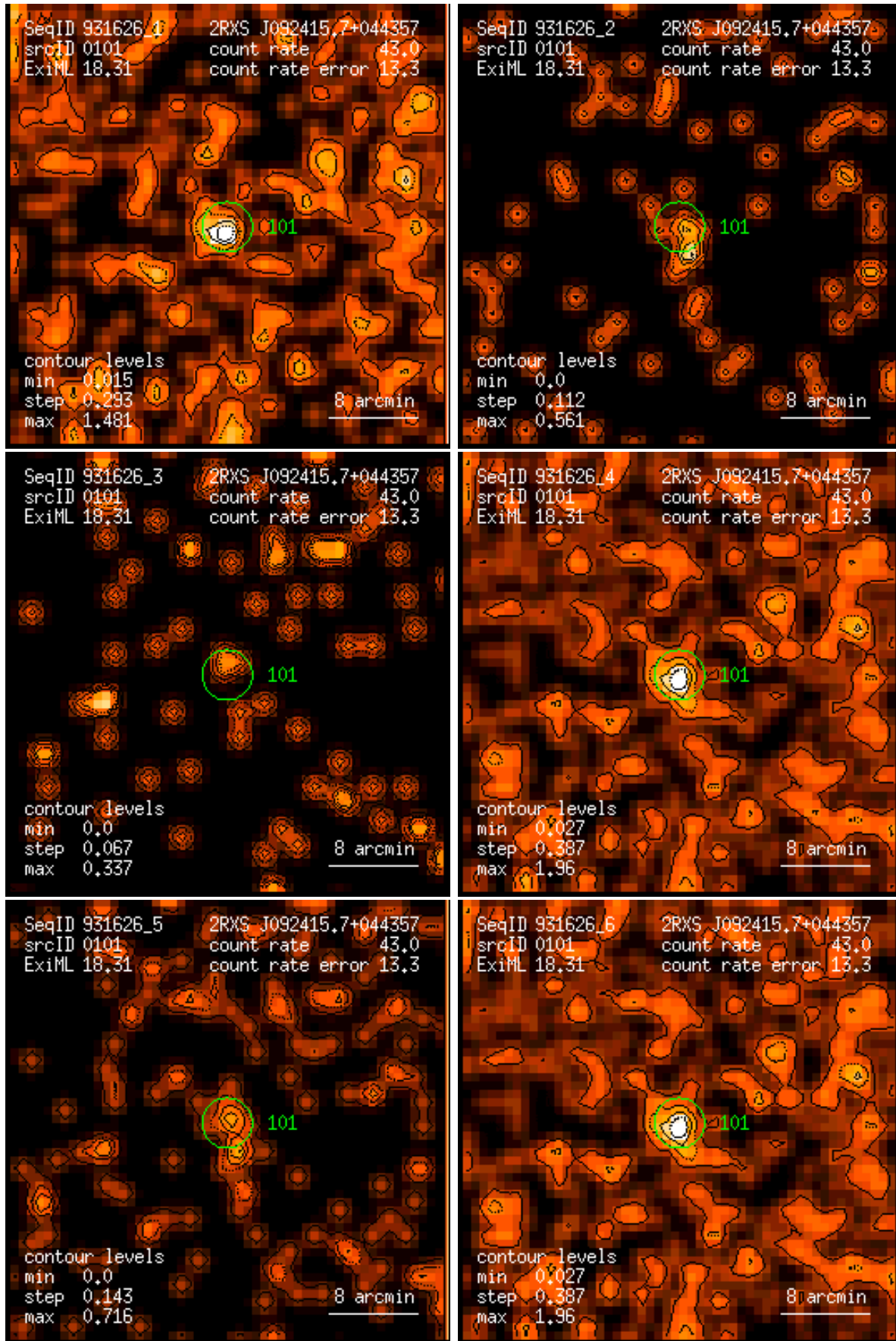
Figure 101: RASS 931626: detection 0101: band rate images, Gaussian filter: (1) PSPC channels 11 – 41, (2) 52 – 90, (3) 91 – 201, (4) 11 – 235, (5) 52 – 201, (6) 11 – 201. Broad band rates in counts/ks. Band rate contour levels in counts/ks/arcmin 2 .
