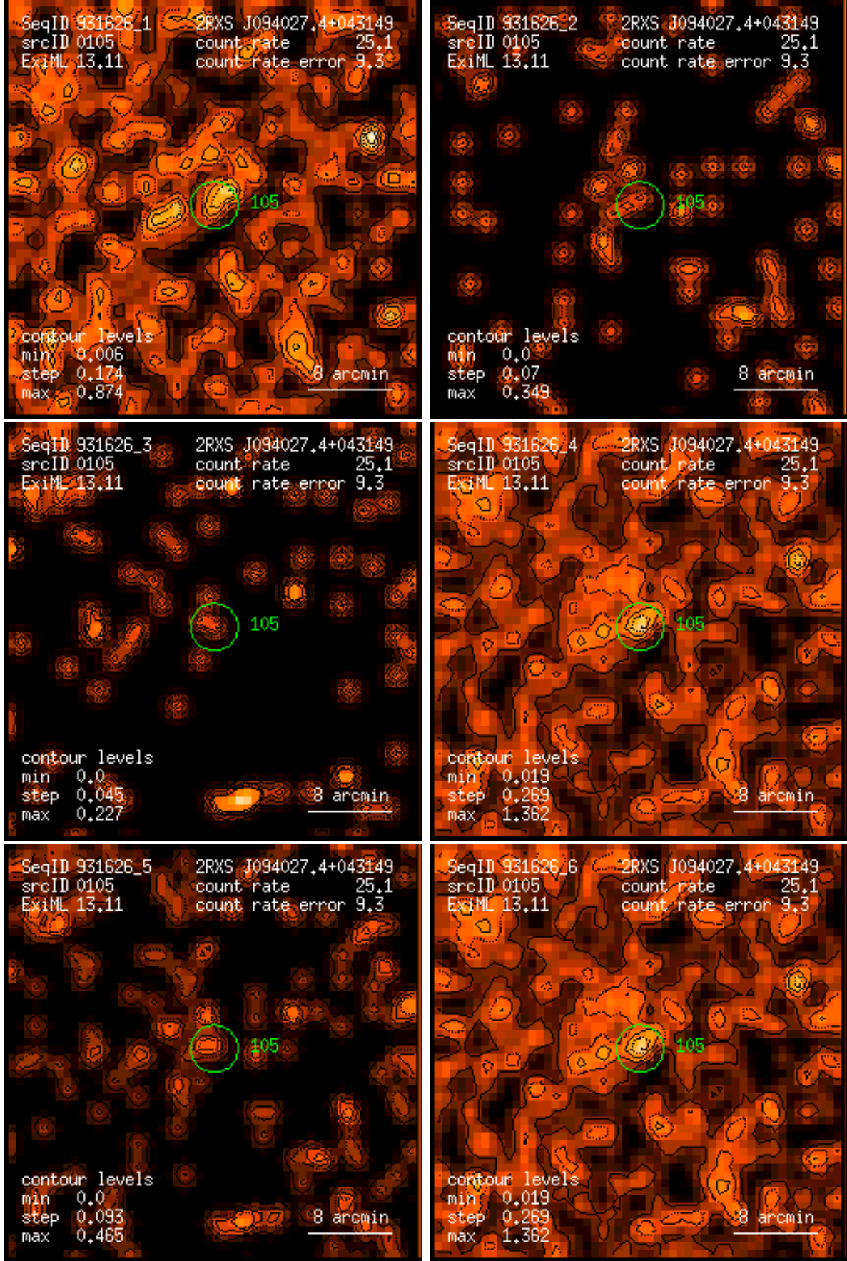
Figure 105: RASS 931626: detection 0105: band rate images, Gaussian filter: (1) PSPC channels 11 – 41, (2) 52 – 90, (3) 91 – 201, (4) 11 – 235, (5) 52 – 201, (6) 11 – 201. Broad band rates in counts/ks. Band rate contour levels in counts/ks/arcmin 2 .
