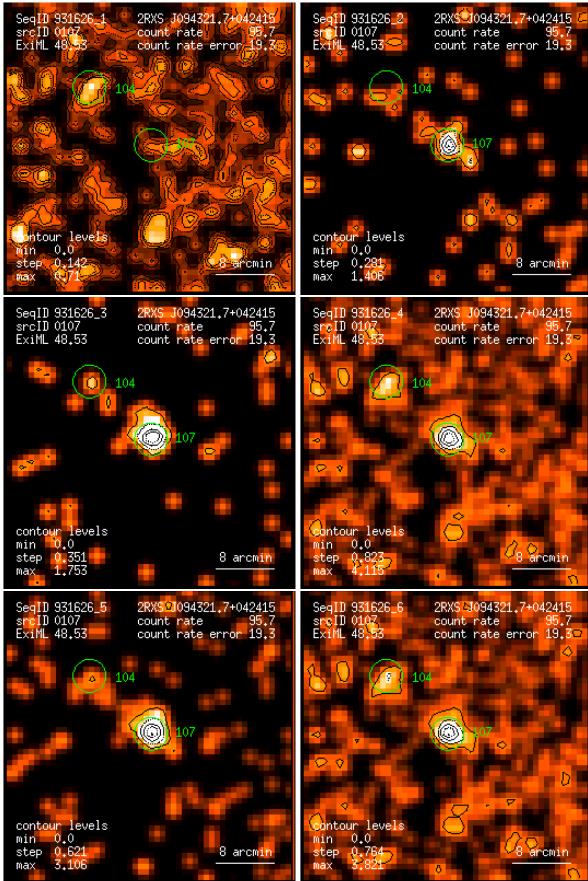
Figure 107: RASS 931626: detection 0107: band rate images, Gaussian filter: (1) PSPC channels 11 – 41, (2) 52 – 90, (3) 91 – 201, (4) 11 – 235, (5) 52 – 201, (6) 11 – 201. Broad band rates in counts/ks. Band rate contour levels in counts/ks/arcmin 2 .
