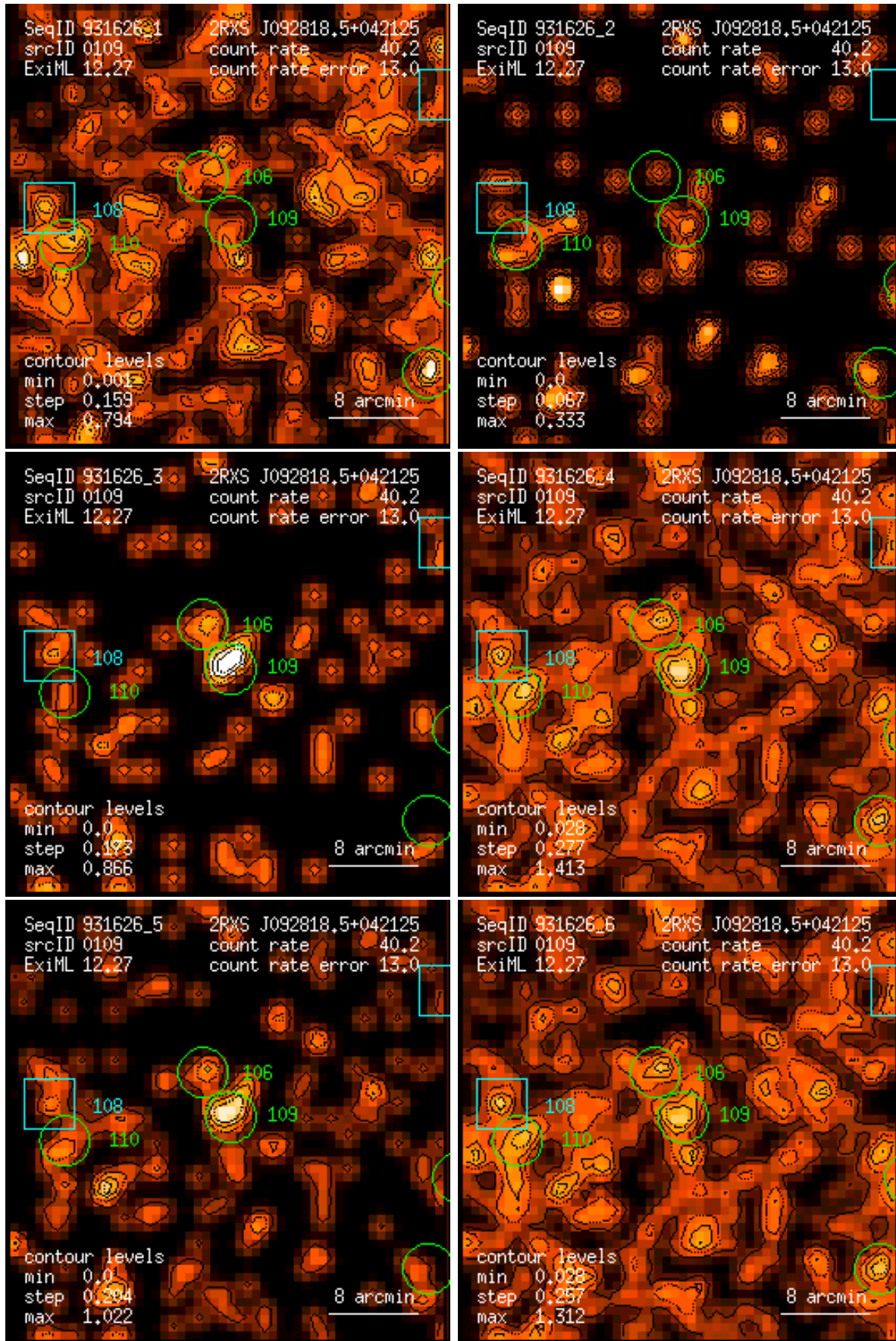
Figure 109: RASS 931626: detection 0109: band rate images, Gaussian filter: (1) PSPC channels 11 – 41, (2) 52 – 90, (3) 91 – 201, (4) 11 – 235, (5) 52 – 201, (6) 11 – 201. Broad band rates in counts/ks. Band rate contour levels in counts/ks/arcmin 2 .
