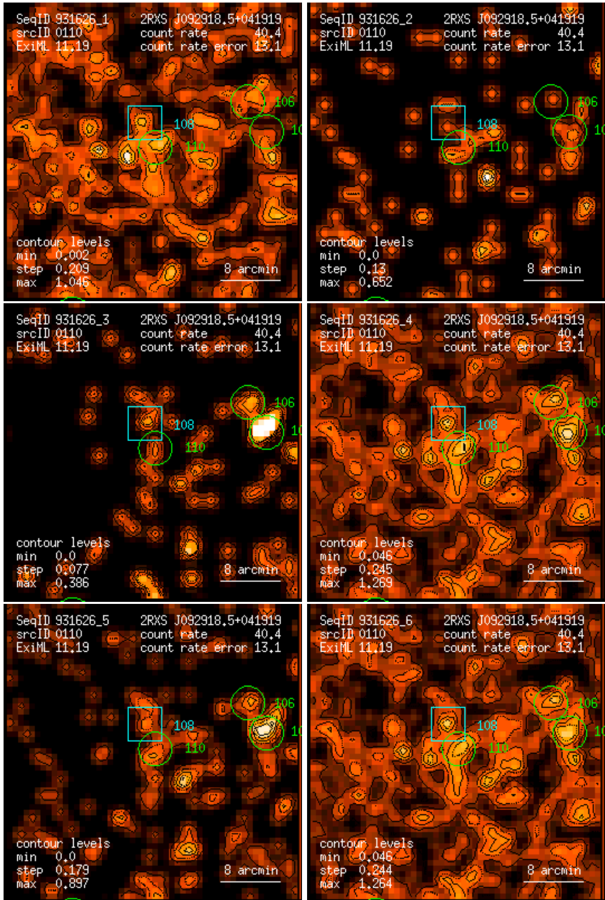
Figure 110: RASS 931626: detection 0110: band rate images, Gaussian filter: (1) PSPC channels 11 – 41, (2) 52 – 90, (3) 91 – 201, (4) 11 – 235, (5) 52 – 201, (6) 11 – 201. Broad band rates in counts/ks. Band rate contour levels in counts/ks/arcmin 2 .
