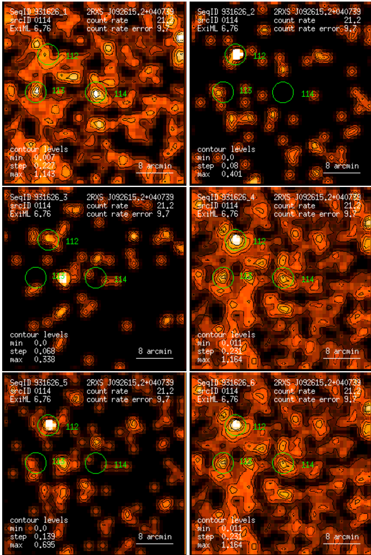
Figure 114: RASS 931626: detection 0114: band rate images, Gaussian filter: (1) PSPC channels 11 – 41, (2) 52 – 90, (3) 91 – 201, (4) 11 – 235, (5) 52 – 201, (6) 11 – 201. Broad band rates in counts/ks. Band rate contour levels in counts/ks/arcmin 2 .
