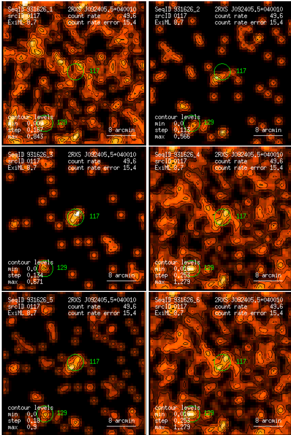
Figure 117: RASS 931626: detection 0117: band rate images, Gaussian filter: (1) PSPC channels 11 – 41, (2) 52 – 90, (3) 91 – 201, (4) 11 – 235, (5) 52 – 201, (6) 11 – 201. Broad band rates in counts/ks. Band rate contour levels in counts/ks/arcmin 2 .
