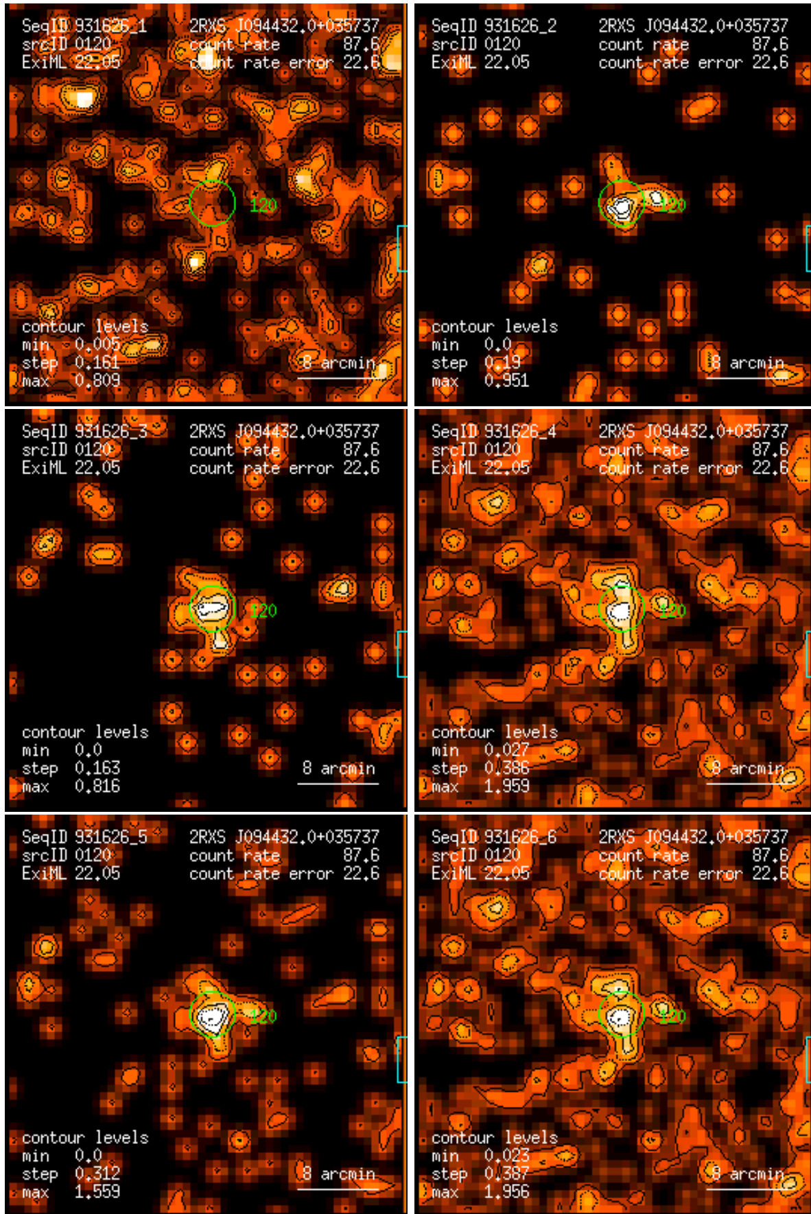
Figure 120: RASS 931626: detection 0120: band rate images, Gaussian filter: (1) PSPC channels 11 – 41, (2) 52 – 90, (3) 91 – 201, (4) 11 – 235, (5) 52 – 201, (6) 11 – 201. Broad band rates in counts/ks. Band rate contour levels in counts/ks/arcmin 2 .
