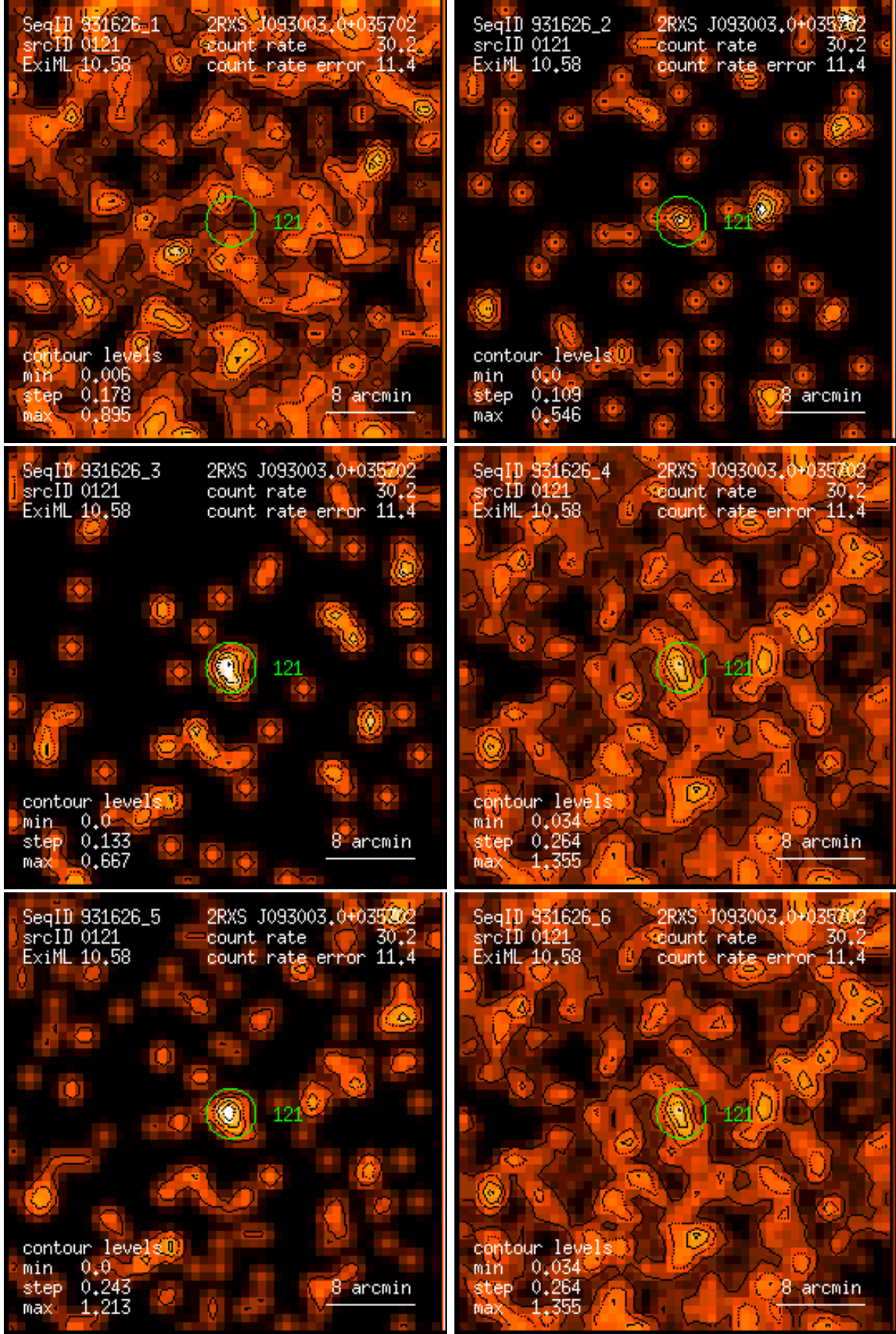
Figure 121: RASS 931626: detection 0121: band rate images, Gaussian filter: (1) PSPC channels 11 – 41, (2) 52 – 90, (3) 91 – 201, (4) 11 – 235, (5) 52 – 201, (6) 11 – 201. Broad band rates in counts/ks. Band rate contour levels in counts/ks/arcmin 2 .
