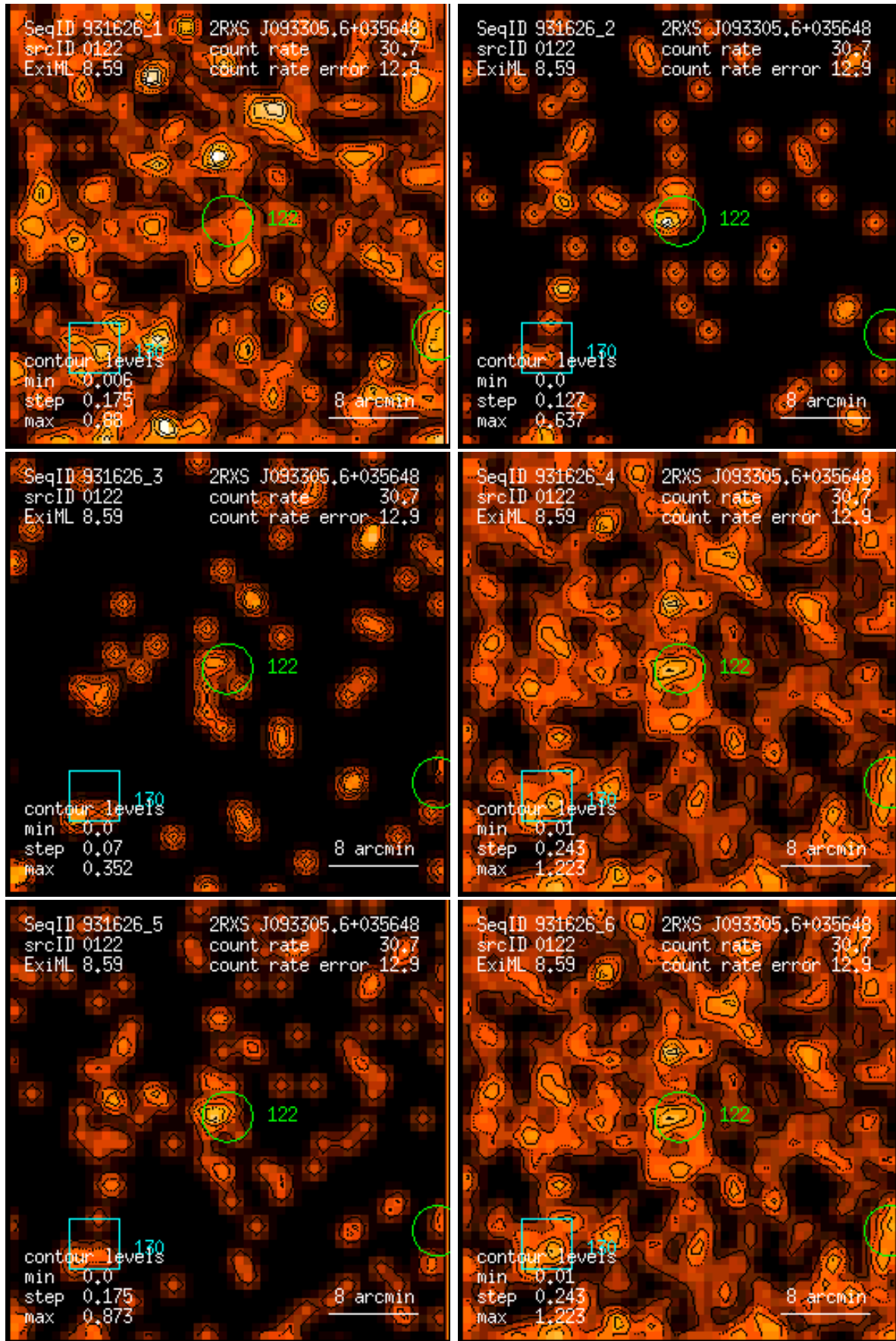
Figure 122: RASS 931626: detection 0122: band rate images, Gaussian filter: (1) PSPC channels 11 – 41, (2) 52 – 90, (3) 91 – 201, (4) 11 – 235, (5) 52 – 201, (6) 11 – 201. Broad band rates in counts/ks. Band rate contour levels in counts/ks/arcmin 2 .
