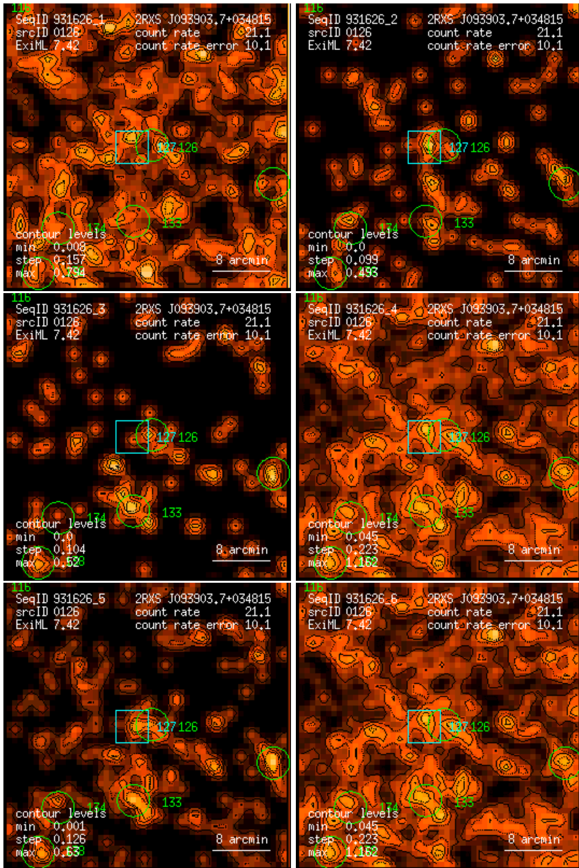
Figure 126: RASS 931626: detection 0126: band rate images, Gaussian filter: (1) PSPC channels 11 – 41, (2) 52 – 90, (3) 91 – 201, (4) 11 – 235, (5) 52 – 201, (6) 11 – 201. Broad band rates in counts/ks. Band rate contour levels in counts/ks/arcmin 2 .
