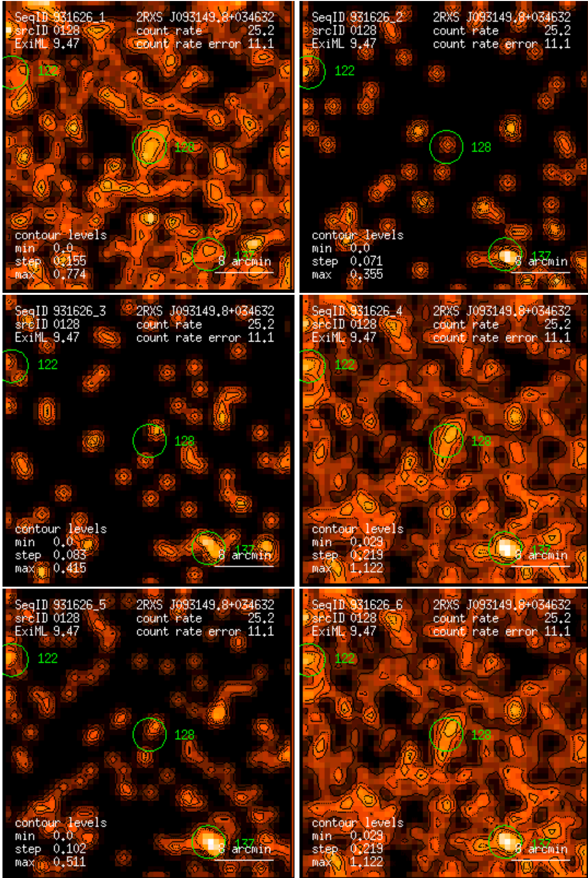
Figure 128: RASS 931626: detection 0128: band rate images, Gaussian filter: (1) PSPC channels 11 – 41, (2) 52 – 90, (3) 91 – 201, (4) 11 – 235, (5) 52 – 201, (6) 11 – 201. Broad band rates in counts/ks. Band rate contour levels in counts/ks/arcmin 2 .
