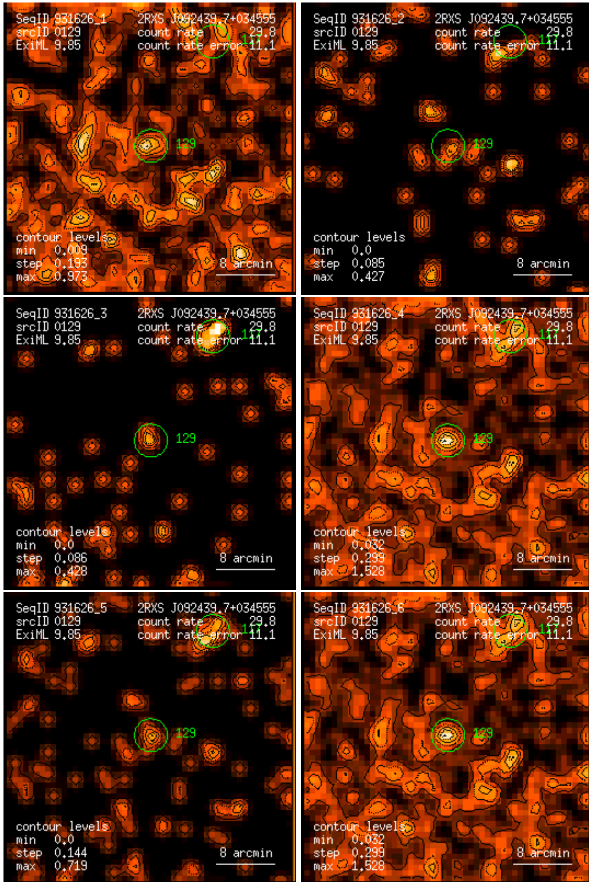
Figure 129: RASS 931626: detection 0129: band rate images, Gaussian filter: (1) PSPC channels 11 – 41, (2) 52 – 90, (3) 91 – 201, (4) 11 – 235, (5) 52 – 201, (6) 11 – 201. Broad band rates in counts/ks. Band rate contour levels in counts/ks/arcmin 2 .
