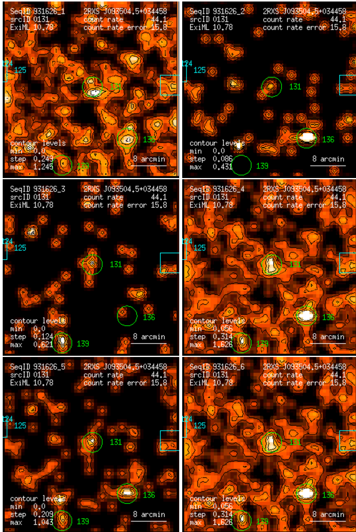
Figure 131: RASS 931626: detection 0131: band rate images, Gaussian filter: (1) PSPC channels 11 – 41, (2) 52 – 90, (3) 91 – 201, (4) 11 – 235, (5) 52 – 201, (6) 11 – 201. Broad band rates in counts/ks. Band rate contour levels in counts/ks/arcmin 2 .
