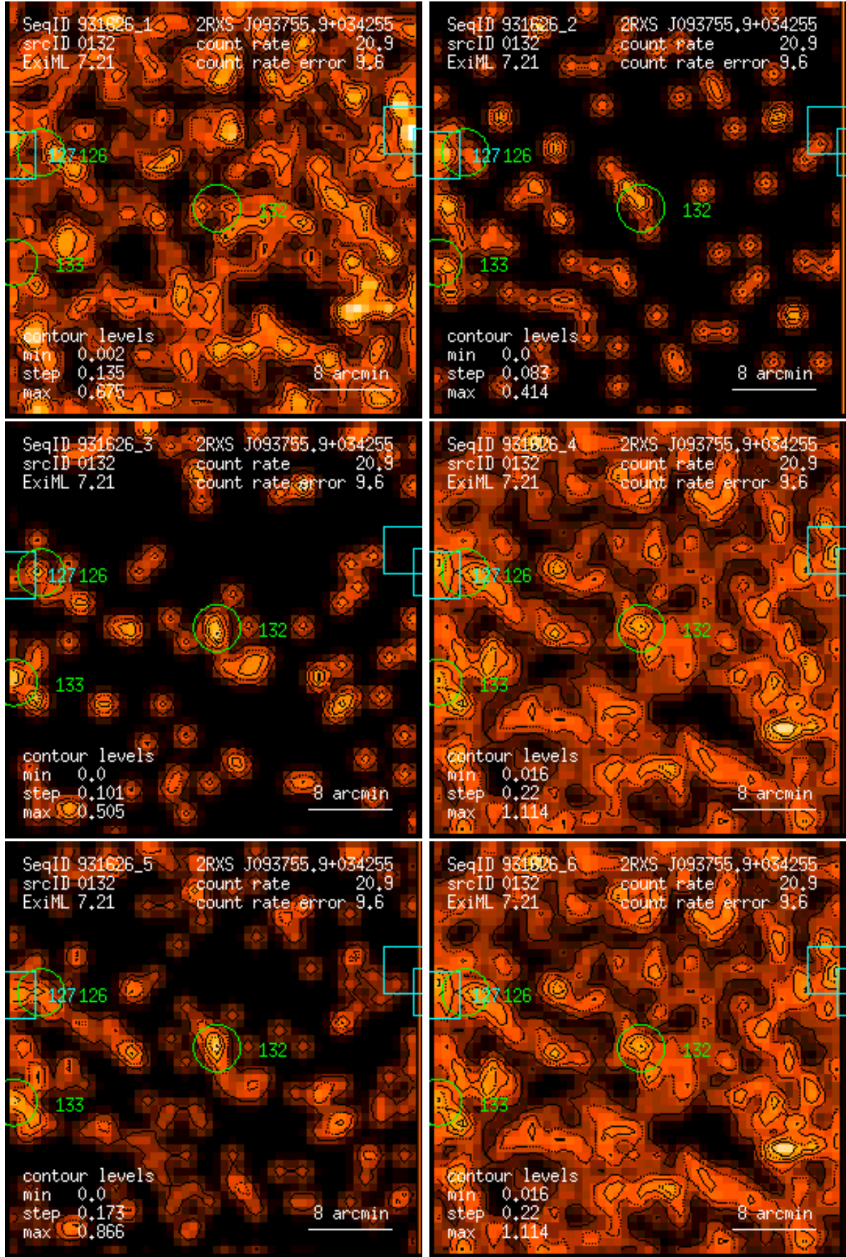
Figure 132: RASS 931626: detection 0132: band rate images, Gaussian filter: (1) PSPC channels 11 – 41, (2) 52 – 90, (3) 91 – 201, (4) 11 – 235, (5) 52 – 201, (6) 11 – 201. Broad band rates in counts/ks. Band rate contour levels in counts/ks/arcmin 2 .
