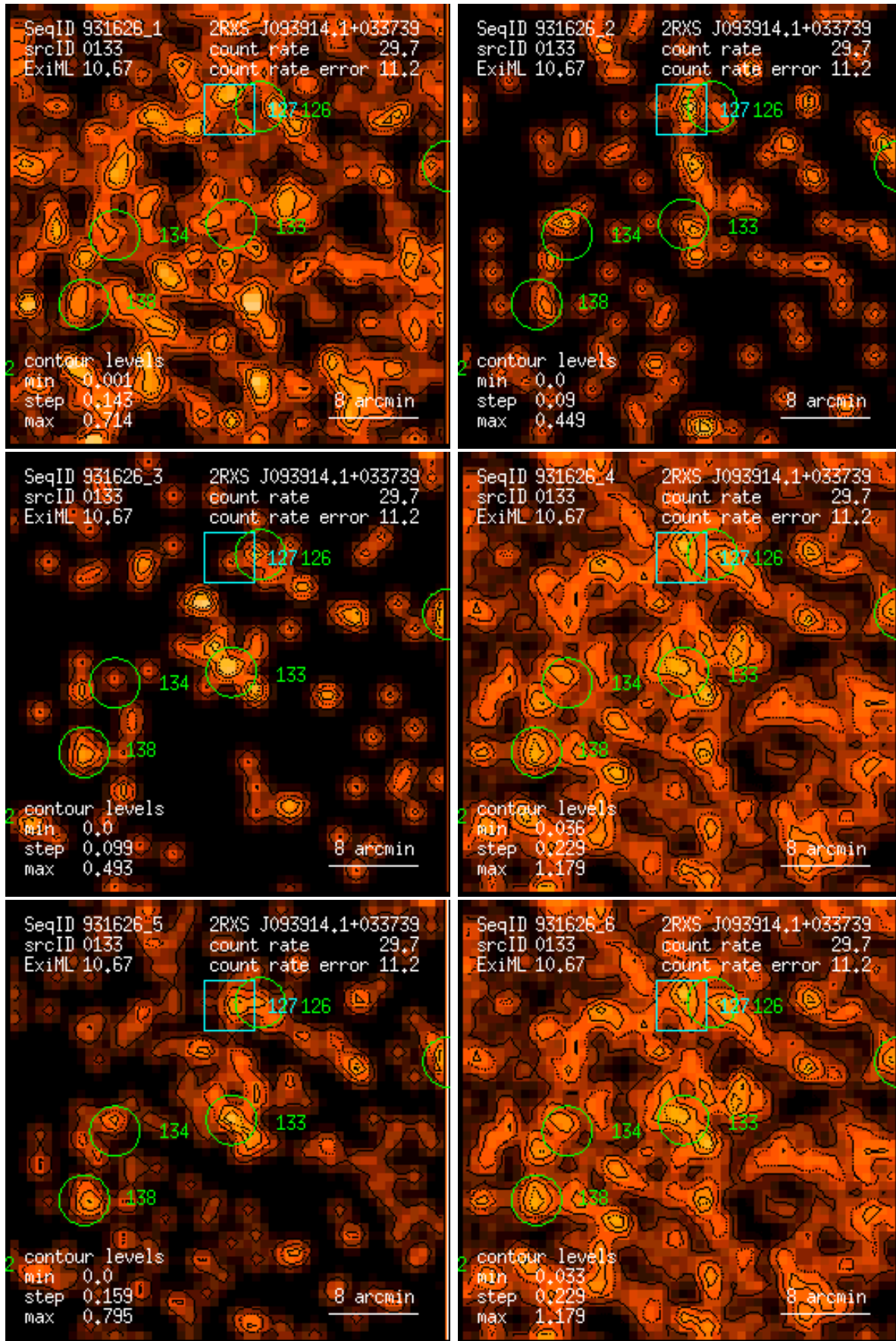
Figure 133: RASS 931626: detection 0133: band rate images, Gaussian filter: (1) PSPC channels 11 – 41, (2) 52 – 90, (3) 91 – 201, (4) 11 – 235, (5) 52 – 201, (6) 11 – 201. Broad band rates in counts/ks. Band rate contour levels in counts/ks/arcmin 2 .
