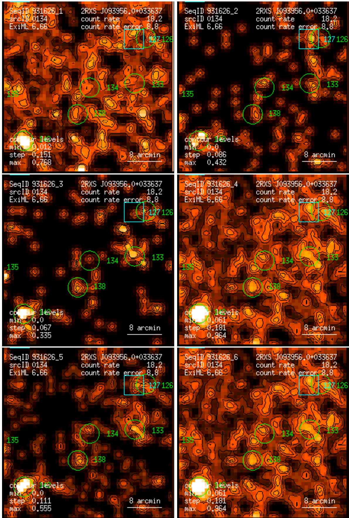
Figure 134: RASS 931626: detection 0134: band rate images, Gaussian filter: (1) PSPC channels 11 – 41, (2) 52 – 90, (3) 91 – 201, (4) 11 – 235, (5) 52 – 201, (6) 11 – 201. Broad band rates in counts/ks. Band rate contour levels in counts/ks/arcmin 2 .
