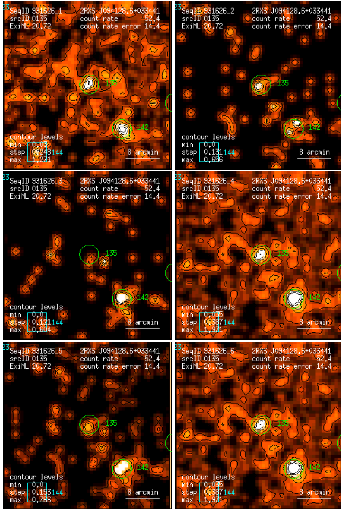
Figure 135: RASS 931626: detection 0135: band rate images, Gaussian filter: (1) PSPC channels 11 – 41, (2) 52 – 90, (3) 91 – 201, (4) 11 – 235, (5) 52 – 201, (6) 11 – 201. Broad band rates in counts/ks. Band rate contour levels in counts/ks/arcmin 2 .
