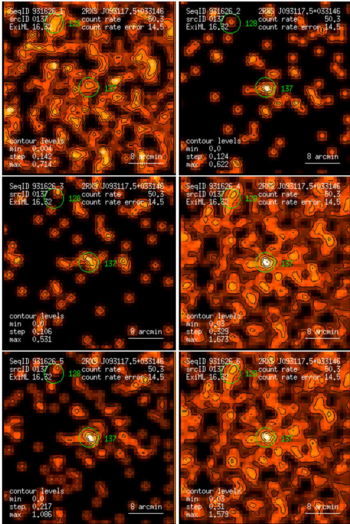
Figure 137: RASS 931626: detection 0137: band rate images, Gaussian filter: (1) PSPC channels 11 – 41, (2) 52 – 90, (3) 91 – 201, (4) 11 – 235, (5) 52 – 201, (6) 11 – 201. Broad band rates in counts/ks. Band rate contour levels in counts/ks/arcmin 2 .
