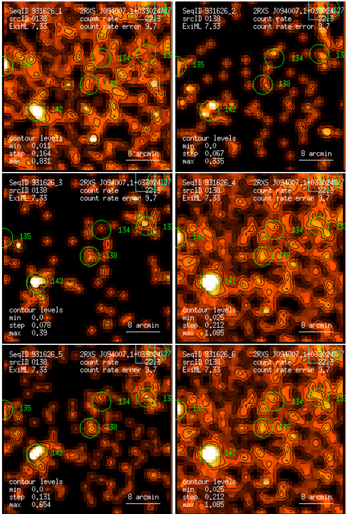
Figure 138: RASS 931626: detection 0138: band rate images, Gaussian filter: (1) PSPC channels 11 – 41, (2) 52 – 90, (3) 91 – 201, (4) 11 – 235, (5) 52 – 201, (6) 11 – 201. Broad band rates in counts/ks. Band rate contour levels in counts/ks/arcmin 2 .
