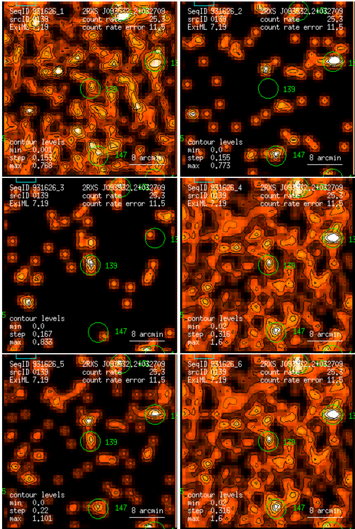
Figure 139: RASS 931626: detection 0139: band rate images, Gaussian filter: (1) PSPC channels 11 – 41, (2) 52 – 90, (3) 91 – 201, (4) 11 – 235, (5) 52 – 201, (6) 11 – 201. Broad band rates in counts/ks. Band rate contour levels in counts/ks/arcmin 2 .
