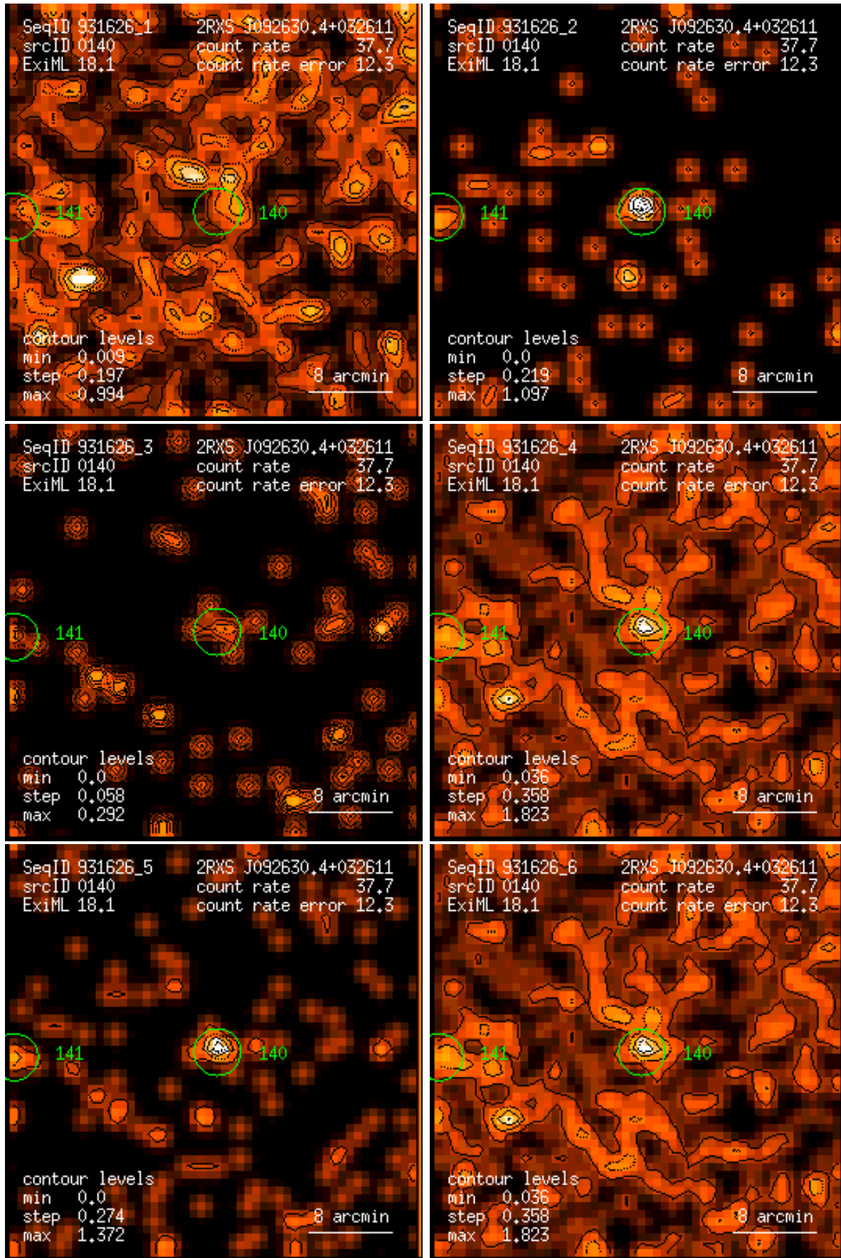
Figure 140: RASS 931626: detection 0140: band rate images, Gaussian filter: (1) PSPC channels 11 – 41, (2) 52 – 90, (3) 91 – 201, (4) 11 – 235, (5) 52 – 201, (6) 11 – 201. Broad band rates in counts/ks. Band rate contour levels in counts/ks/arcmin 2 .
