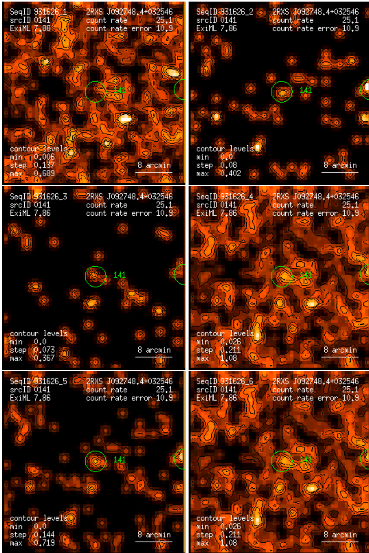
Figure 141: RASS 931626: detection 0141: band rate images, Gaussian filter: (1) PSPC channels 11 – 41, (2) 52 – 90, (3) 91 – 201, (4) 11 – 235, (5) 52 – 201, (6) 11 – 201. Broad band rates in counts/ks. Band rate contour levels in counts/ks/arcmin 2 .
