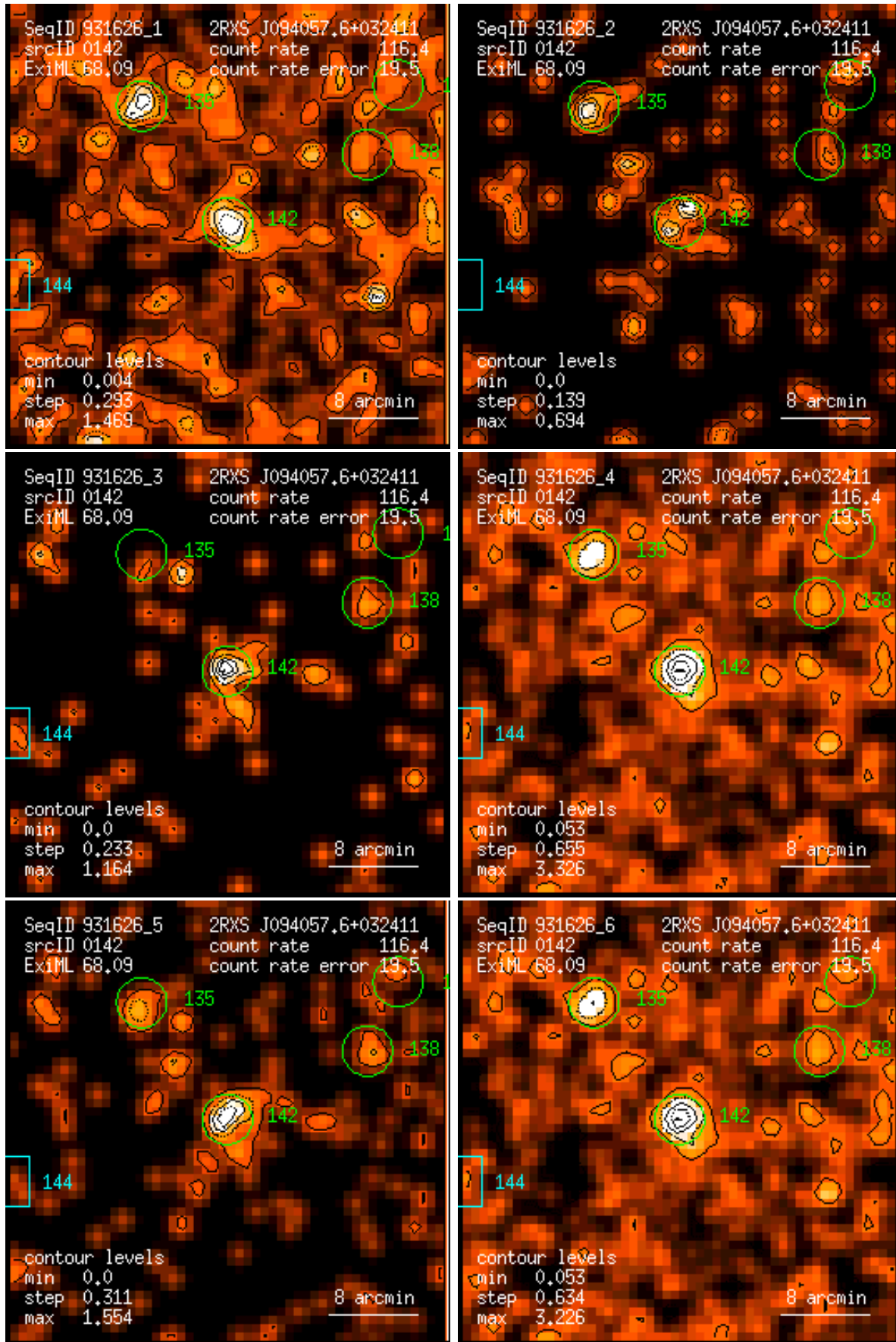
Figure 142: RASS 931626: detection 0142: band rate images, Gaussian filter: (1) PSPC channels 11 – 41, (2) 52 – 90, (3) 91 – 201, (4) 11 – 235, (5) 52 – 201, (6) 11 – 201. Broad band rates in counts/ks. Band rate contour levels in counts/ks/arcmin 2 .
