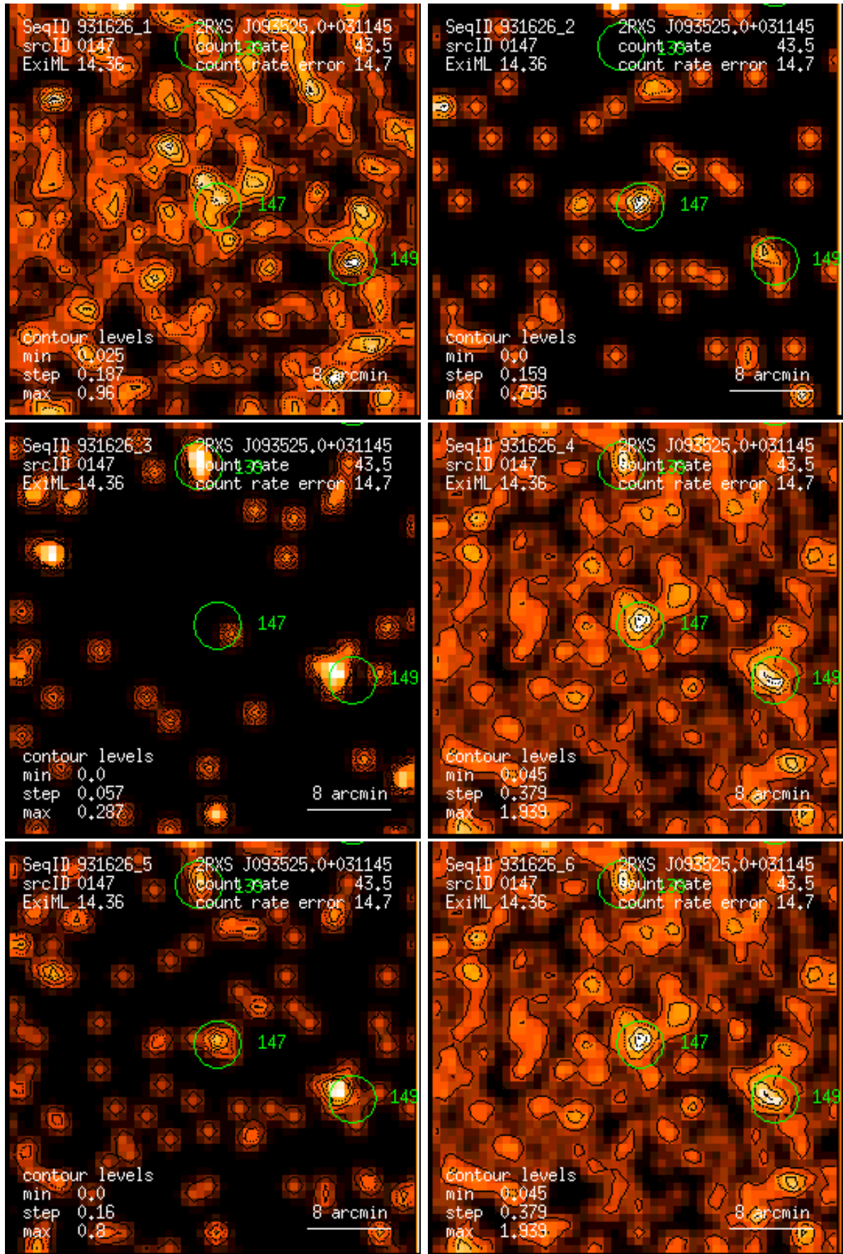
Figure 147: RASS 931626: detection 0147: band rate images, Gaussian filter: (1) PSPC channels 11 – 41, (2) 52 – 90, (3) 91 – 201, (4) 11 – 235, (5) 52 – 201, (6) 11 – 201. Broad band rates in counts/ks. Band rate contour levels in counts/ks/arcmin 2 .
