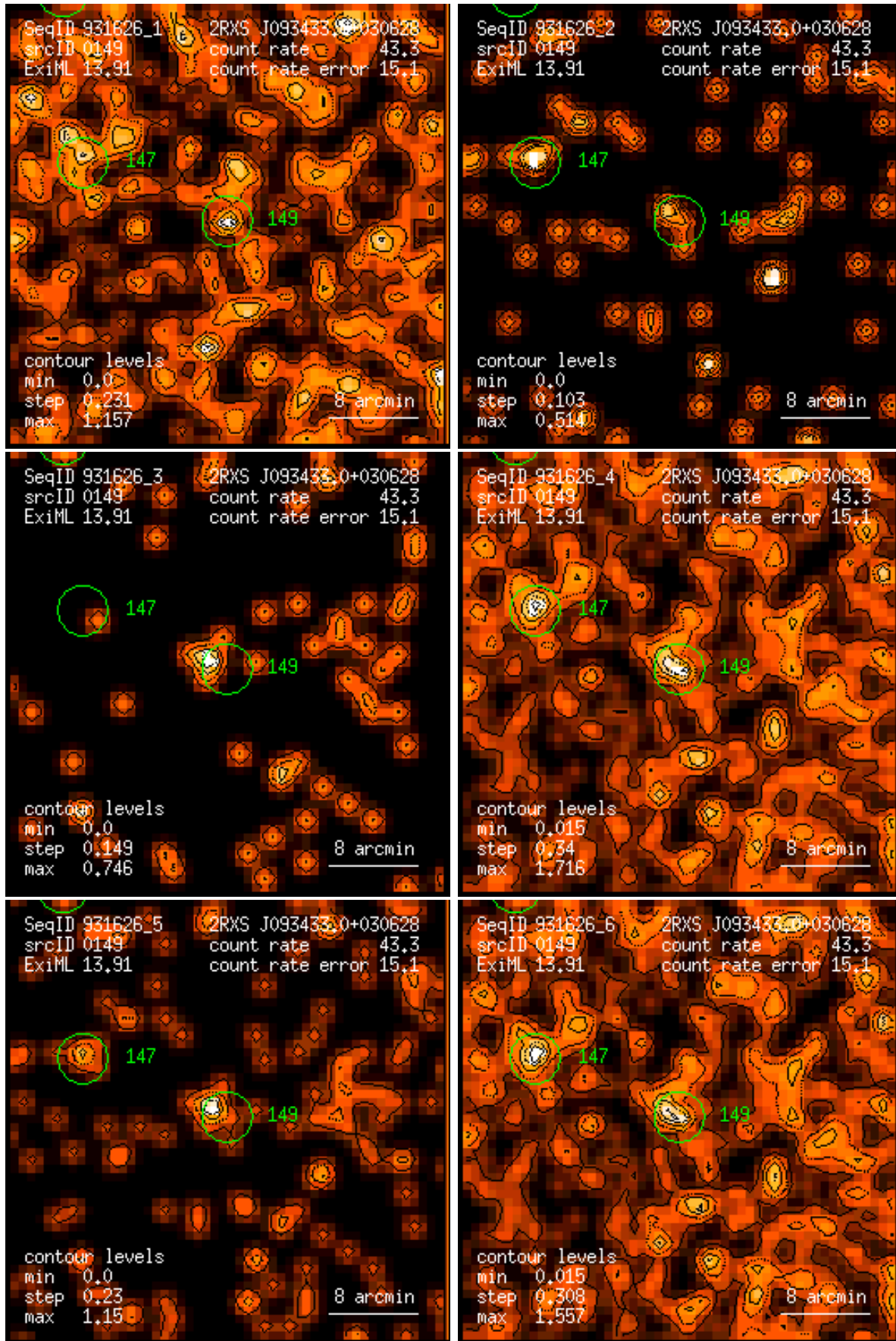
Figure 149: RASS 931626: detection 0149: band rate images, Gaussian filter: (1) PSPC channels 11 – 41, (2) 52 – 90, (3) 91 – 201, (4) 11 – 235, (5) 52 – 201, (6) 11 – 201. Broad band rates in counts/ks. Band rate contour levels in counts/ks/arcmin 2 .
