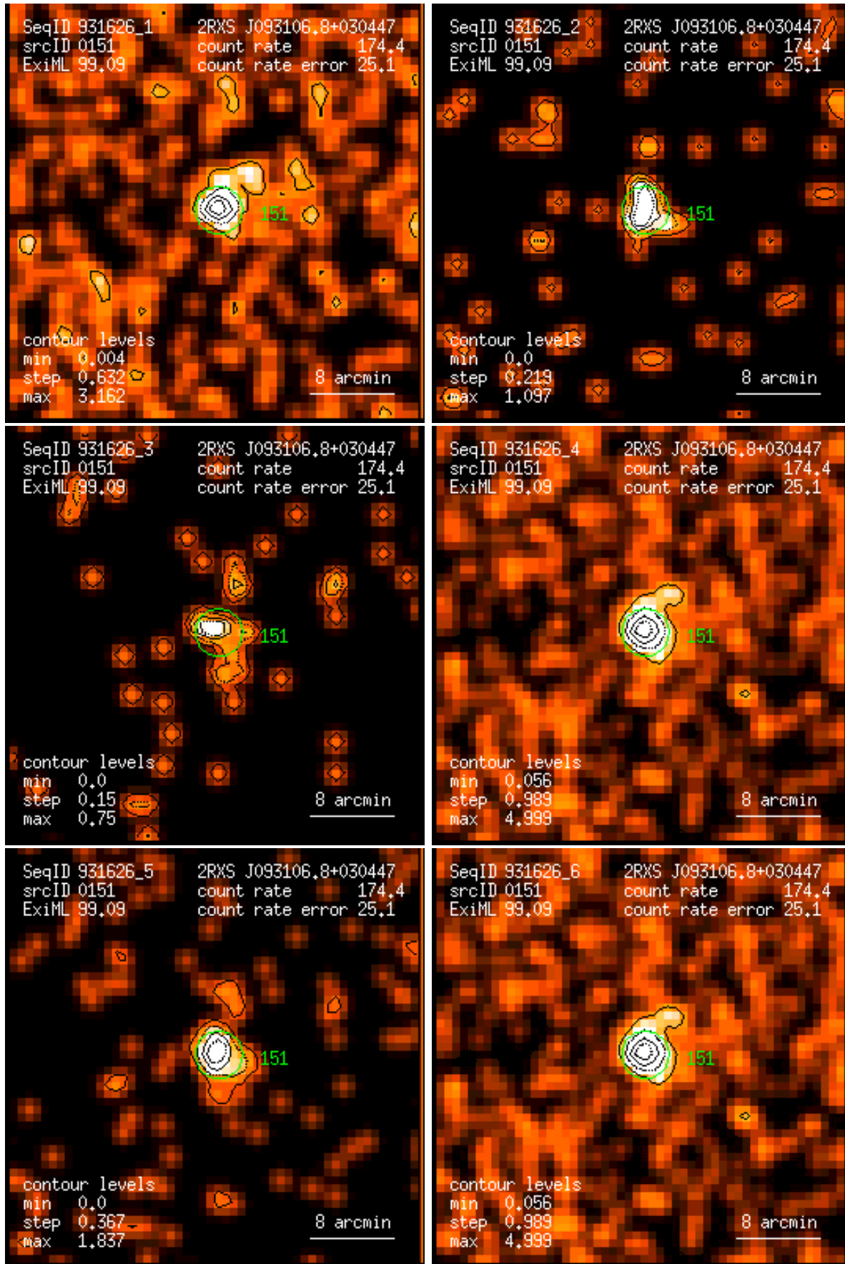
Figure 151: RASS 931626: detection 0151: band rate images, Gaussian filter: (1) PSPC channels 11 – 41, (2) 52 – 90, (3) 91 – 201, (4) 11 – 235, (5) 52 – 201, (6) 11 – 201. Broad band rates in counts/ks. Band rate contour levels in counts/ks/arcmin 2 .
