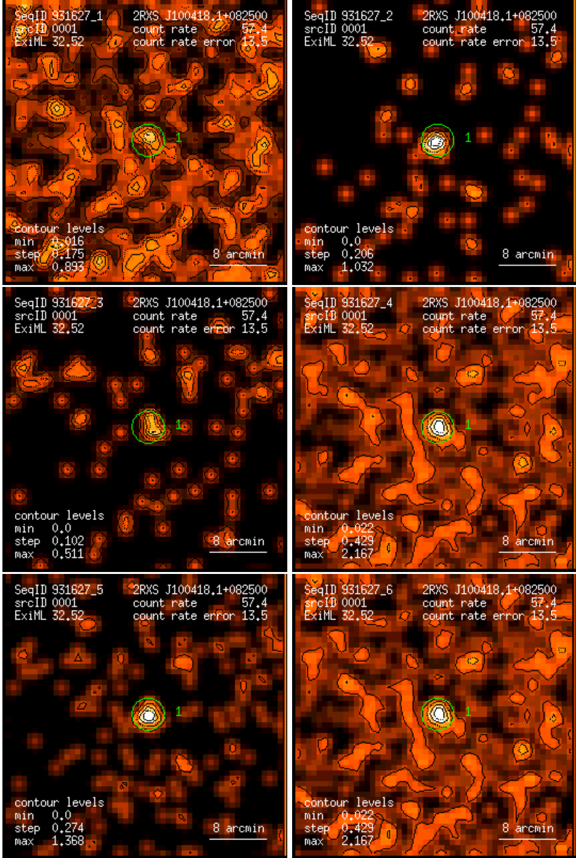
Figure 1: RASS 931627: detection 0001: band rate images, Gaussian filter: (1) PSPC channels 11 – 41, (2) 52 – 90, (3) 91 – 201, (4) 11 – 235, (5) 52 – 201, (6) 11 – 201. Broad band rates in counts/ks. Band rate contour levels in counts/ks/arcmin 2 .
