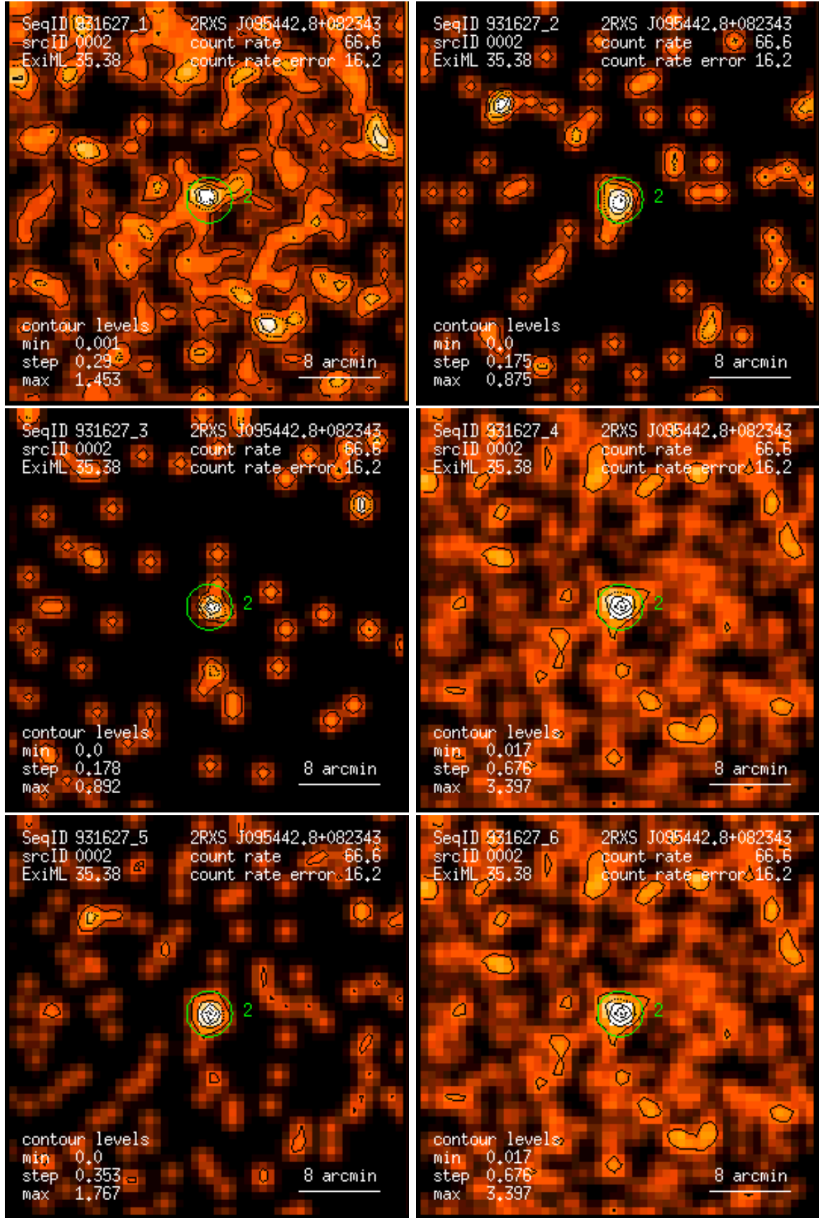
Figure 2: RASS 931627: detection 0002: band rate images, Gaussian filter: (1) PSPC channels 11 – 41, (2) 52 – 90, (3) 91 – 201, (4) 11 – 235, (5) 52 – 201, (6) 11 – 201. Broad band rates in counts/ks. Band rate contour levels in counts/ks/arcmin 2 .
