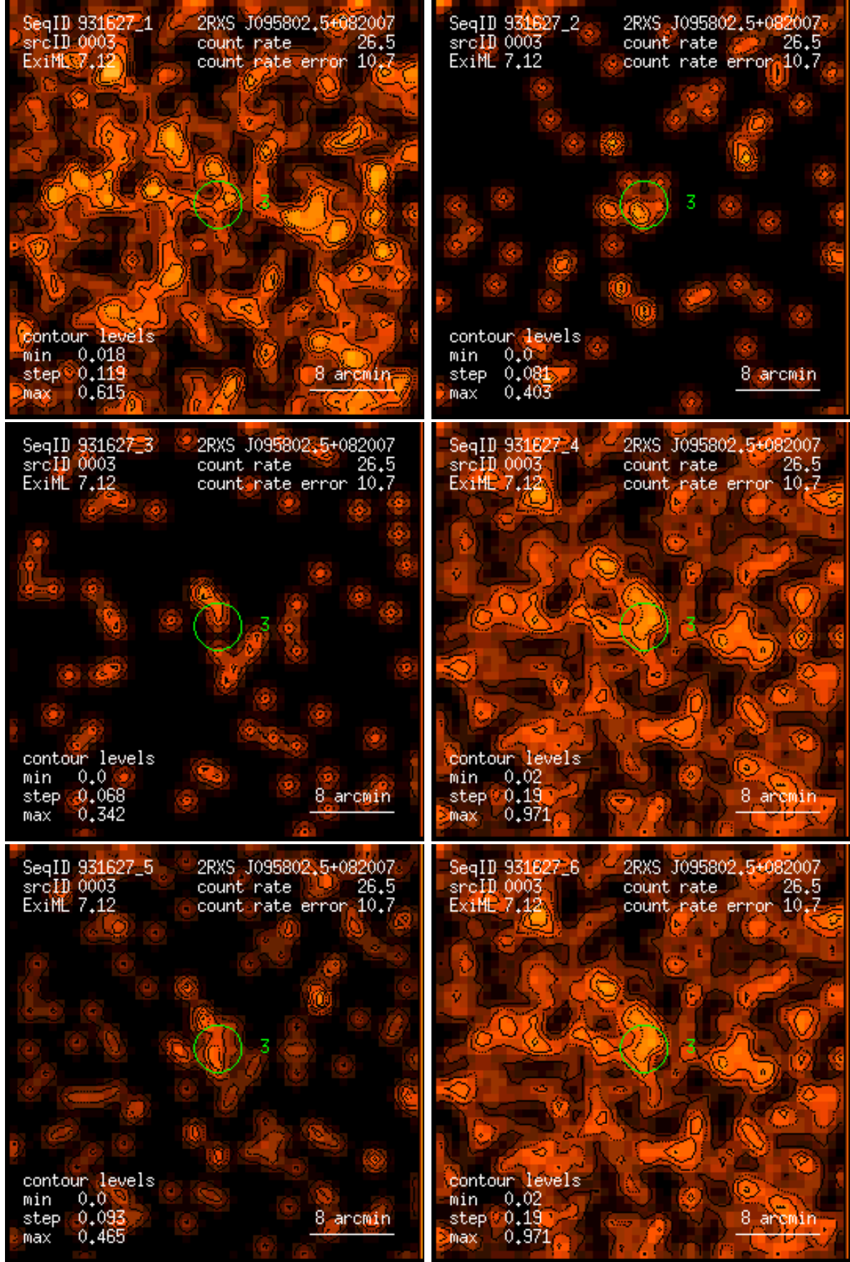
Figure 3: RASS 931627: detection 0003: band rate images, Gaussian filter: (1) PSPC channels 11 – 41, (2) 52 – 90, (3) 91 – 201, (4) 11 – 235, (5) 52 – 201, (6) 11 – 201. Broad band rates in counts/ks. Band rate contour levels in counts/ks/arcmin 2 .
