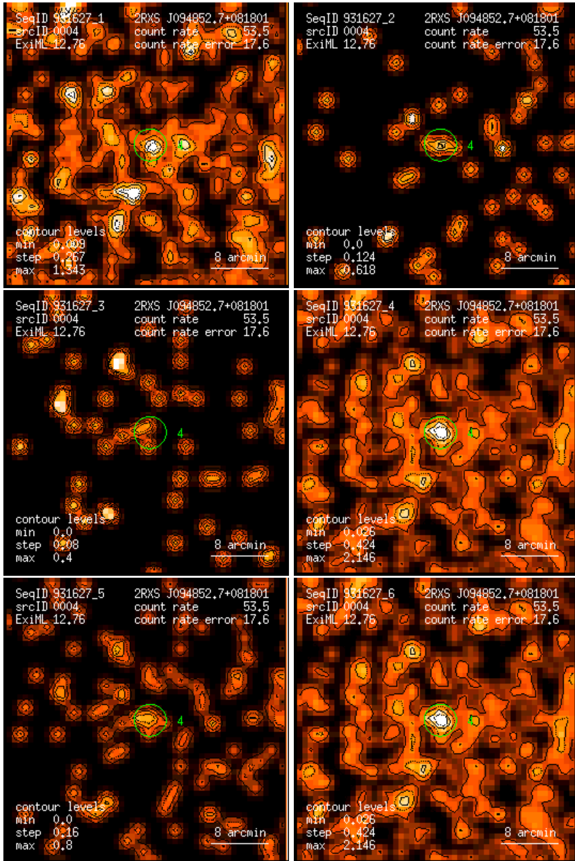
Figure 4: RASS 931627: detection 0004: band rate images, Gaussian filter: (1) PSPC channels 11 – 41, (2) 52 – 90, (3) 91 – 201, (4) 11 – 235, (5) 52 – 201, (6) 11 – 201. Broad band rates in counts/ks. Band rate contour levels in counts/ks/arcmin 2 .
