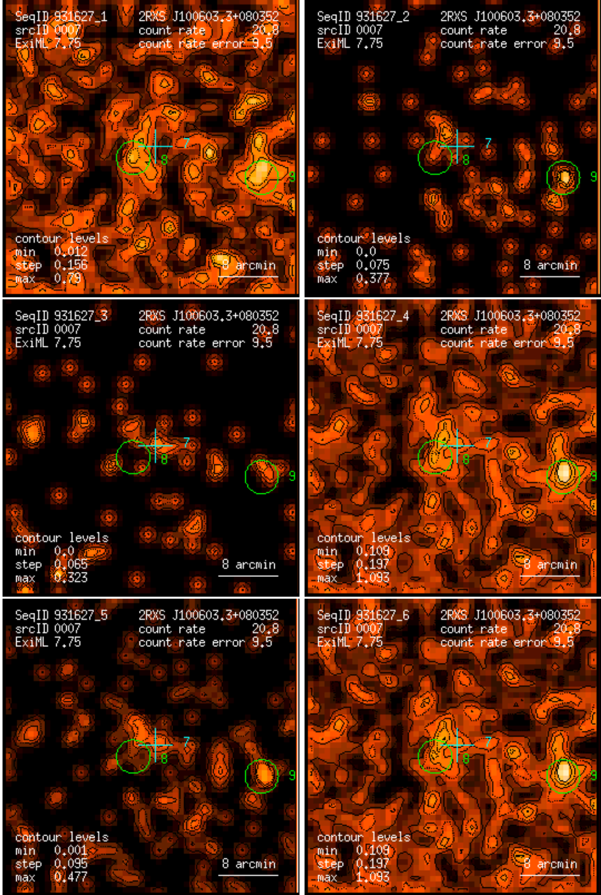
Figure 7: RASS 931627: detection 0007: band rate images, Gaussian filter: (1) PSPC channels 11 – 41, (2) 52 – 90, (3) 91 – 201, (4) 11 – 235, (5) 52 – 201, (6) 11 – 201. Broad band rates in counts/ks. Band rate contour levels in counts/ks/arcmin 2 .
