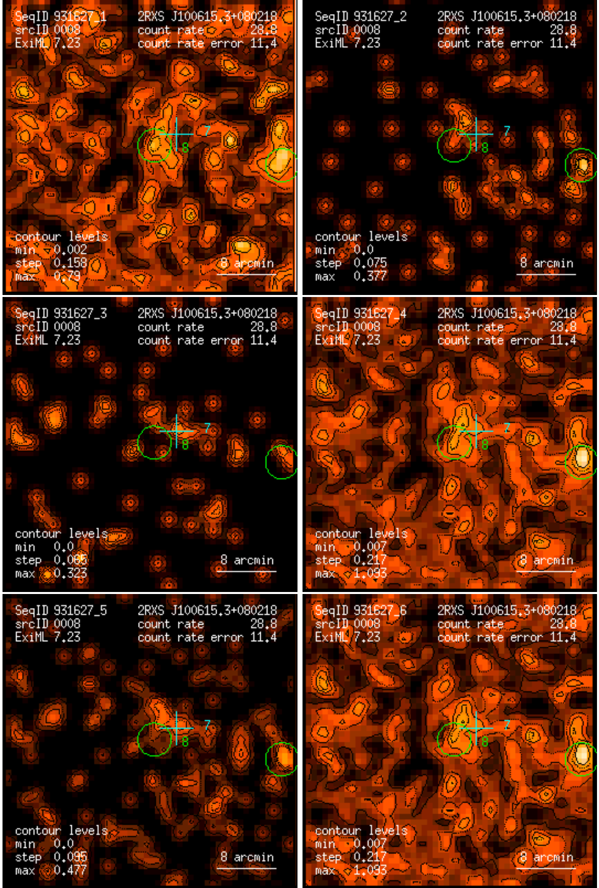
Figure 8: RASS 931627: detection 0008: band rate images, Gaussian filter: (1) PSPC channels 11 – 41, (2) 52 – 90, (3) 91 – 201, (4) 11 – 235, (5) 52 – 201, (6) 11 – 201. Broad band rates in counts/ks. Band rate contour levels in counts/ks/arcmin 2 .
