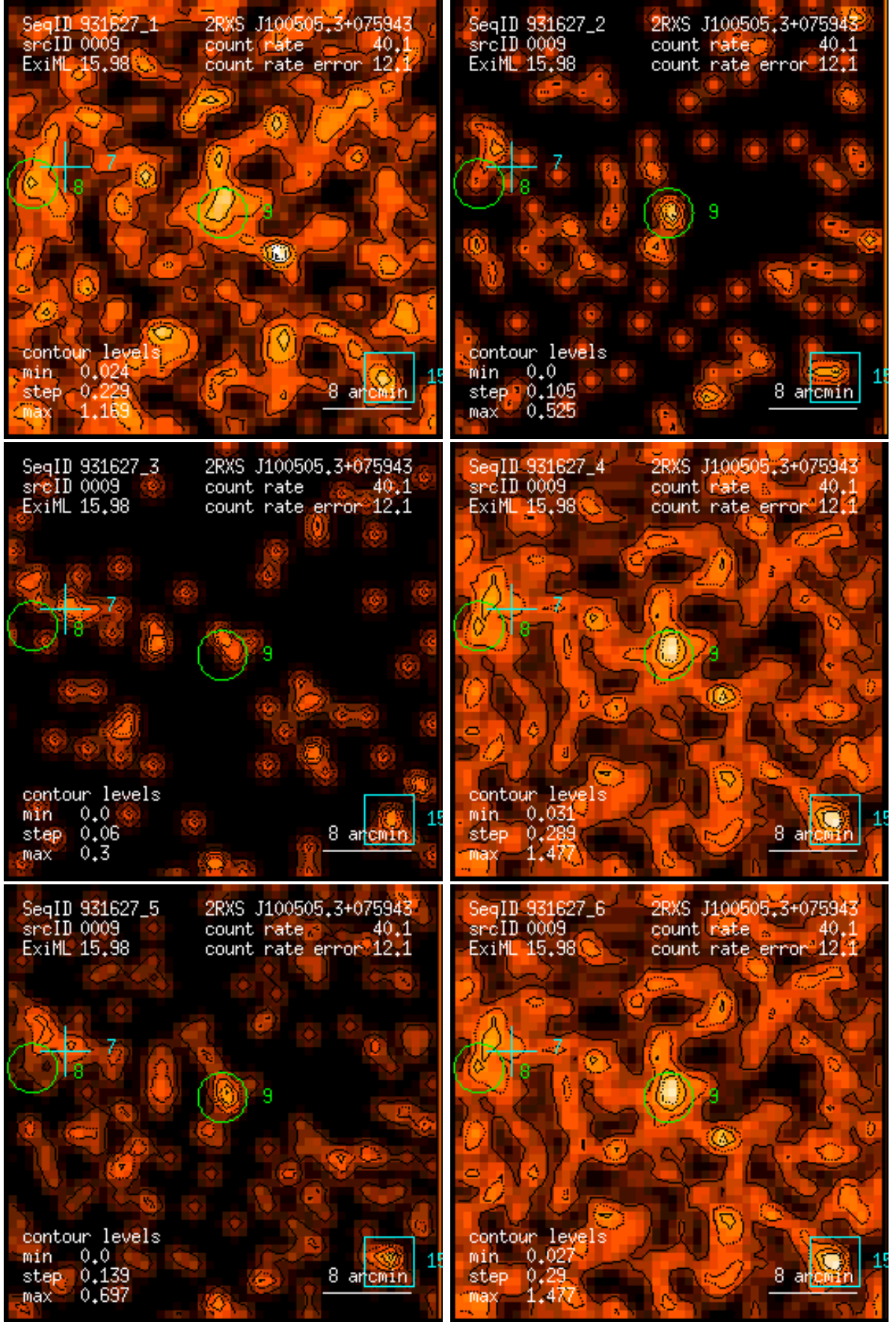
Figure 9: RASS 931627: detection 0009: band rate images, Gaussian filter: (1) PSPC channels 11 – 41, (2) 52 – 90, (3) 91 – 201, (4) 11 – 235, (5) 52 – 201, (6) 11 – 201. Broad band rates in counts/ks. Band rate contour levels in counts/ks/arcmin 2 .
