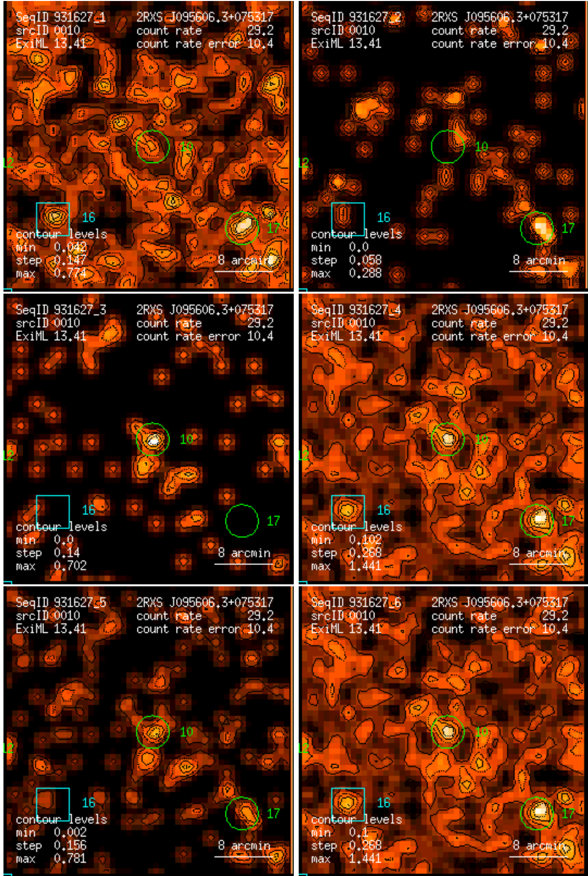
Figure 10: RASS 931627: detection 0010: band rate images, Gaussian filter: (1) PSPC channels 11 – 41, (2) 52 – 90, (3) 91 – 201, (4) 11 – 235, (5) 52 – 201, (6) 11 – 201. Broad band rates in counts/ks. Band rate contour levels in counts/ks/arcmin 2 .
