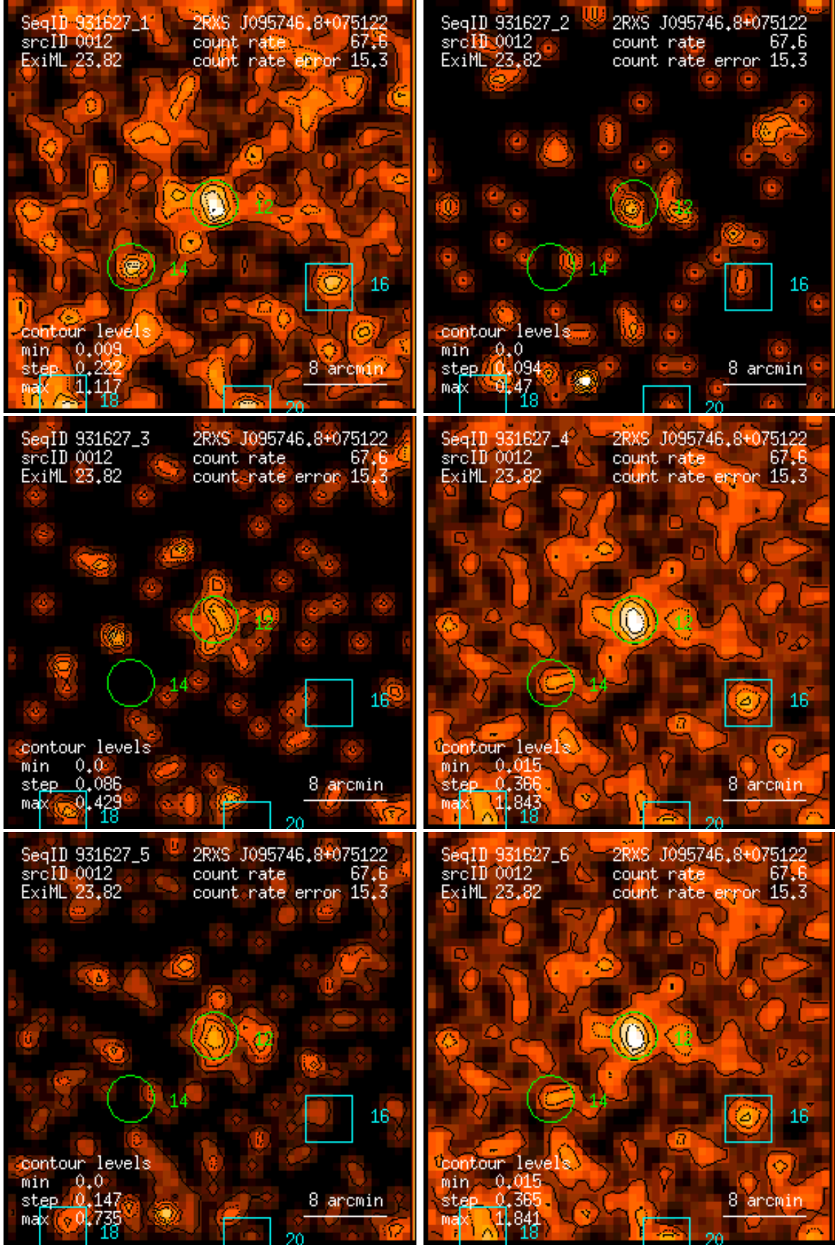
Figure 12: RASS 931627: detection 0012: band rate images, Gaussian filter: (1) PSPC channels 11 – 41, (2) 52 – 90, (3) 91 – 201, (4) 11 – 235, (5) 52 – 201, (6) 11 – 201. Broad band rates in counts/ks. Band rate contour levels in counts/ks/arcmin 2 .
