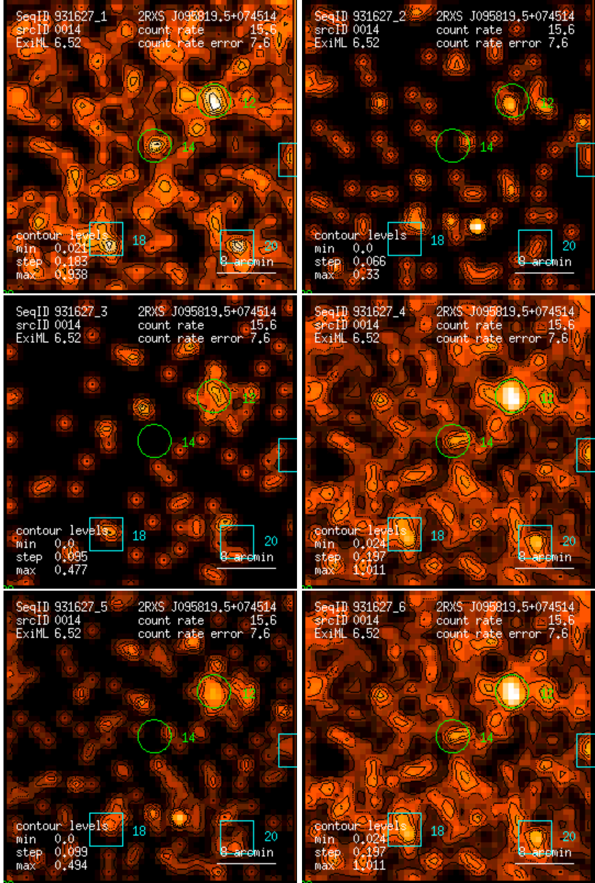
Figure 14: RASS 931627: detection 0014: band rate images, Gaussian filter: (1) PSPC channels 11 – 41, (2) 52 – 90, (3) 91 – 201, (4) 11 – 235, (5) 52 – 201, (6) 11 – 201. Broad band rates in counts/ks. Band rate contour levels in counts/ks/arcmin 2 .
