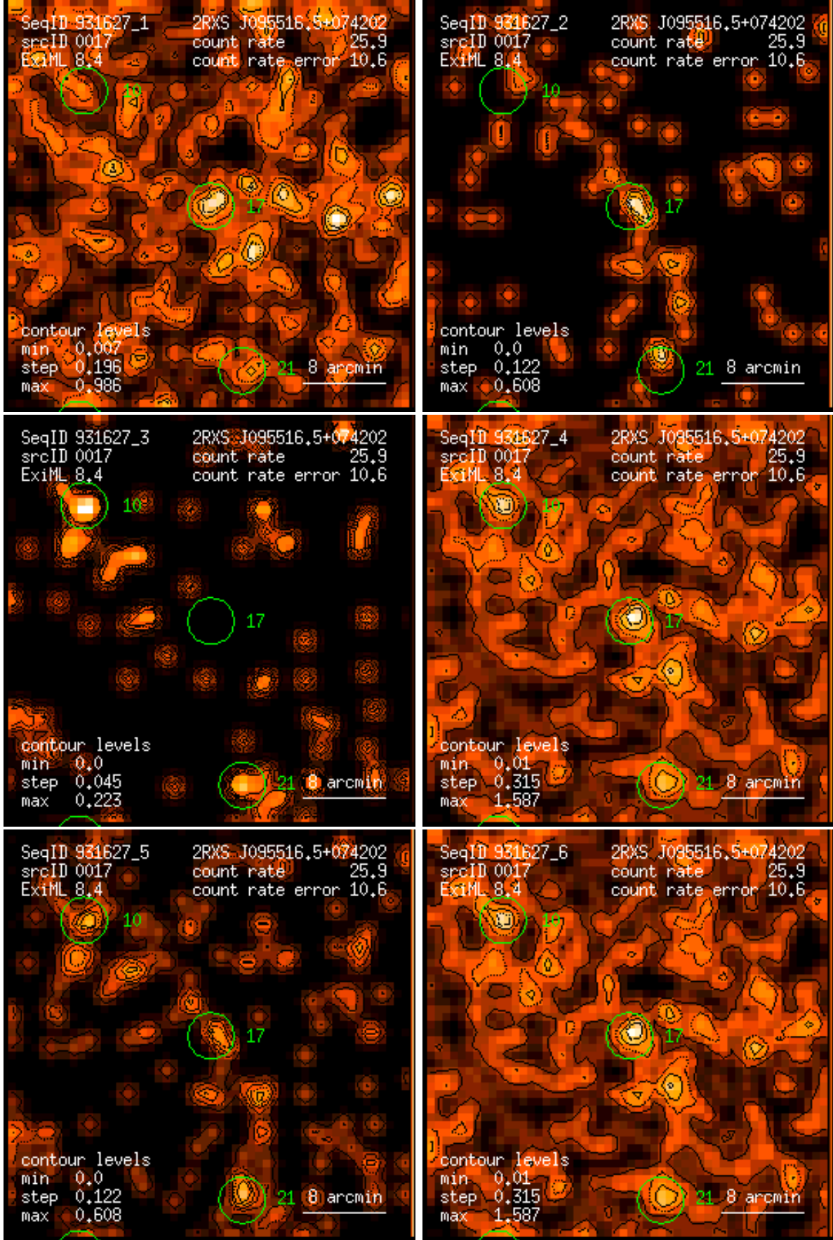
Figure 17: RASS 931627: detection 0017: band rate images, Gaussian filter: (1) PSPC channels 11 – 41, (2) 52 – 90, (3) 91 – 201, (4) 11 – 235, (5) 52 – 201, (6) 11 – 201. Broad band rates in counts/ks. Band rate contour levels in counts/ks/arcmin 2 .
