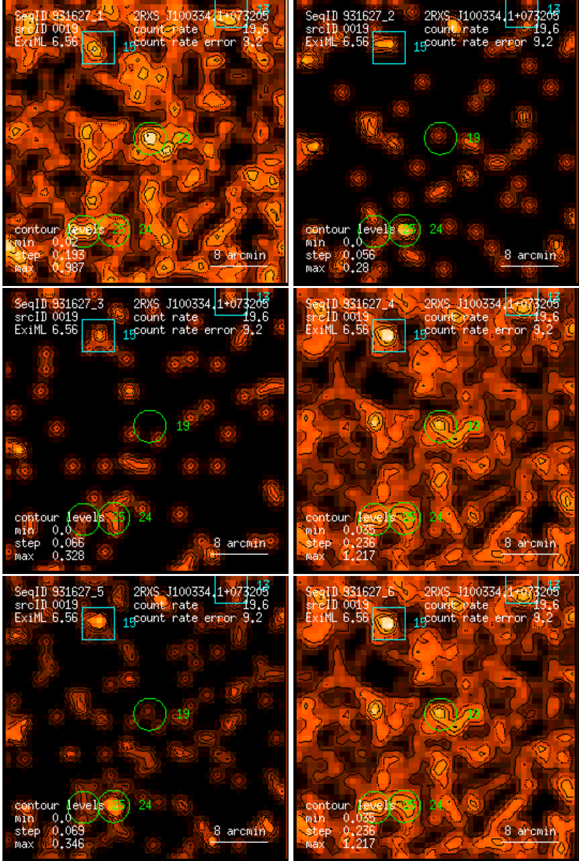
Figure 19: RASS 931627: detection 0019: band rate images, Gaussian filter: (1) PSPC channels 11 – 41, (2) 52 – 90, (3) 91 – 201, (4) 11 – 235, (5) 52 – 201, (6) 11 – 201. Broad band rates in counts/ks. Band rate contour levels in counts/ks/arcmin 2 .
