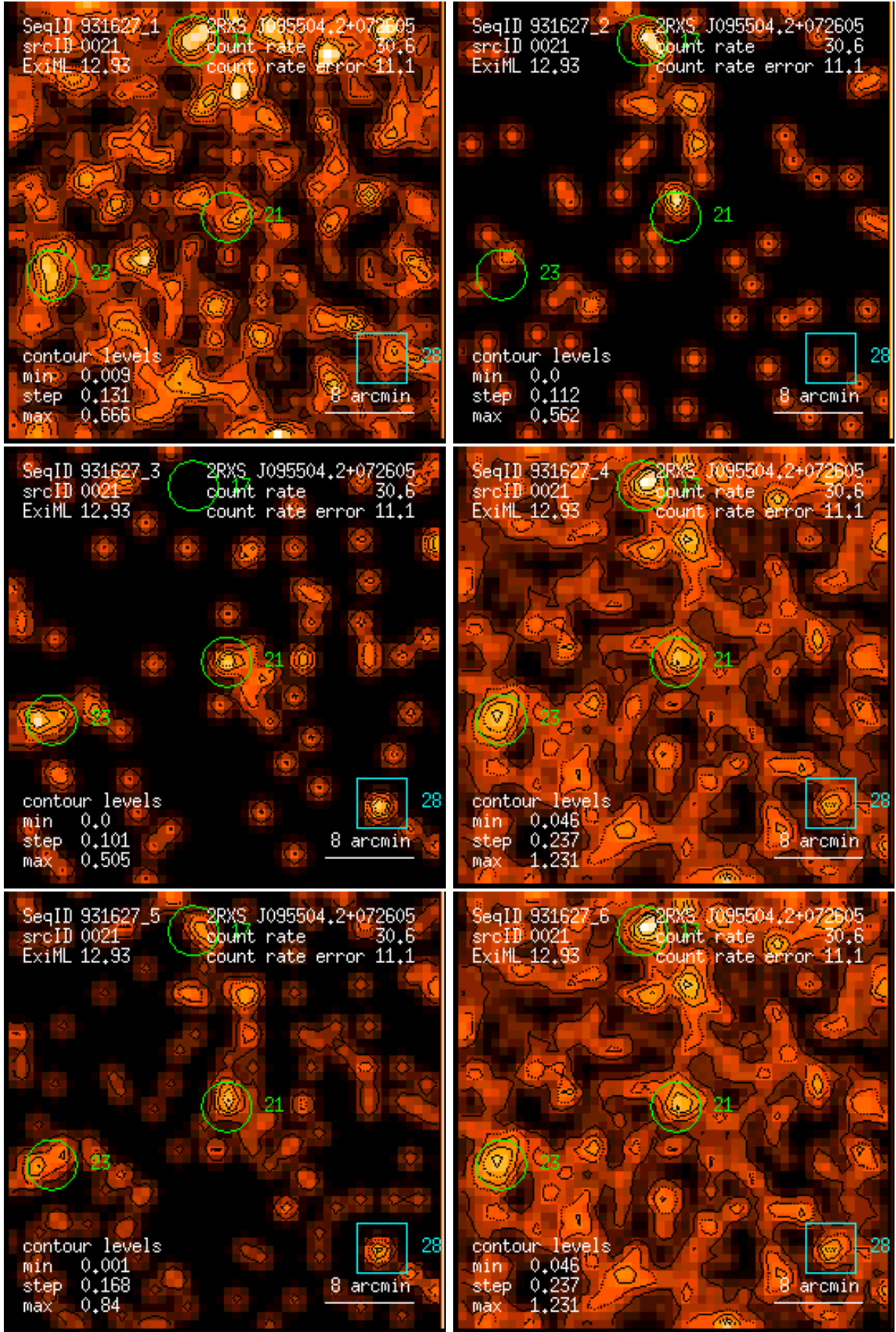
Figure 21: RASS 931627: detection 0021: band rate images, Gaussian filter: (1) PSPC channels 11 – 41, (2) 52 – 90, (3) 91 – 201, (4) 11 – 235, (5) 52 – 201, (6) 11 – 201. Broad band rates in counts/ks. Band rate contour levels in counts/ks/arcmin 2 .
