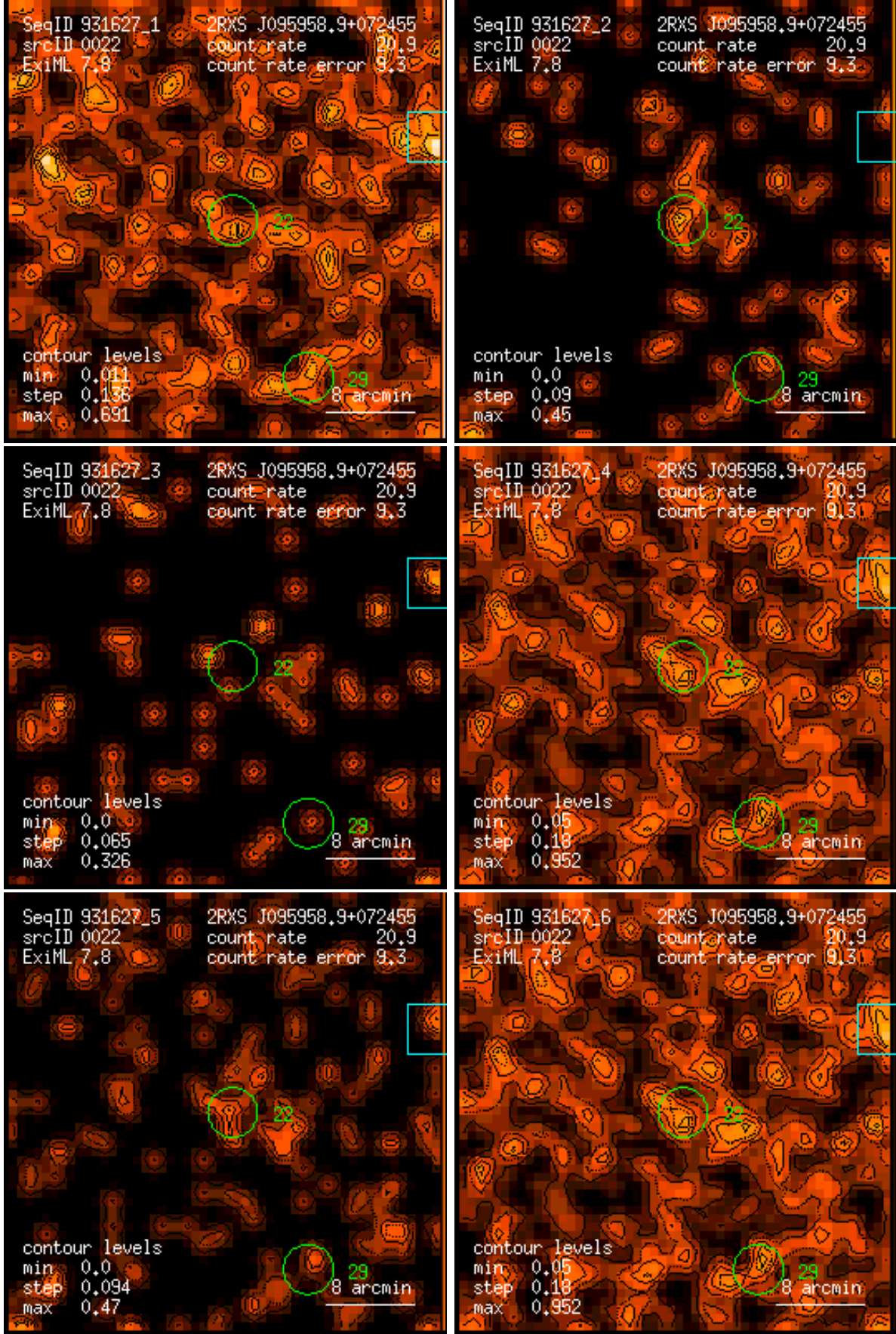
Figure 22: RASS 931627: detection 0022: band rate images, Gaussian filter: (1) PSPC channels 11 – 41, (2) 52 – 90, (3) 91 – 201, (4) 11 – 235, (5) 52 – 201, (6) 11 – 201. Broad band rates in counts/ks. Band rate contour levels in counts/ks/arcmin 2 .
