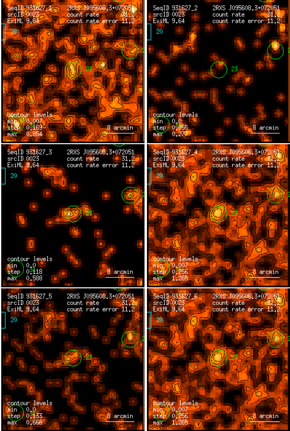
Figure 23: RASS 931627: detection 0023: band rate images, Gaussian filter: (1) PSPC channels 11 – 41, (2) 52 – 90, (3) 91 – 201, (4) 11 – 235, (5) 52 – 201, (6) 11 – 201. Broad band rates in counts/ks. Band rate contour levels in counts/ks/arcmin 2 .
