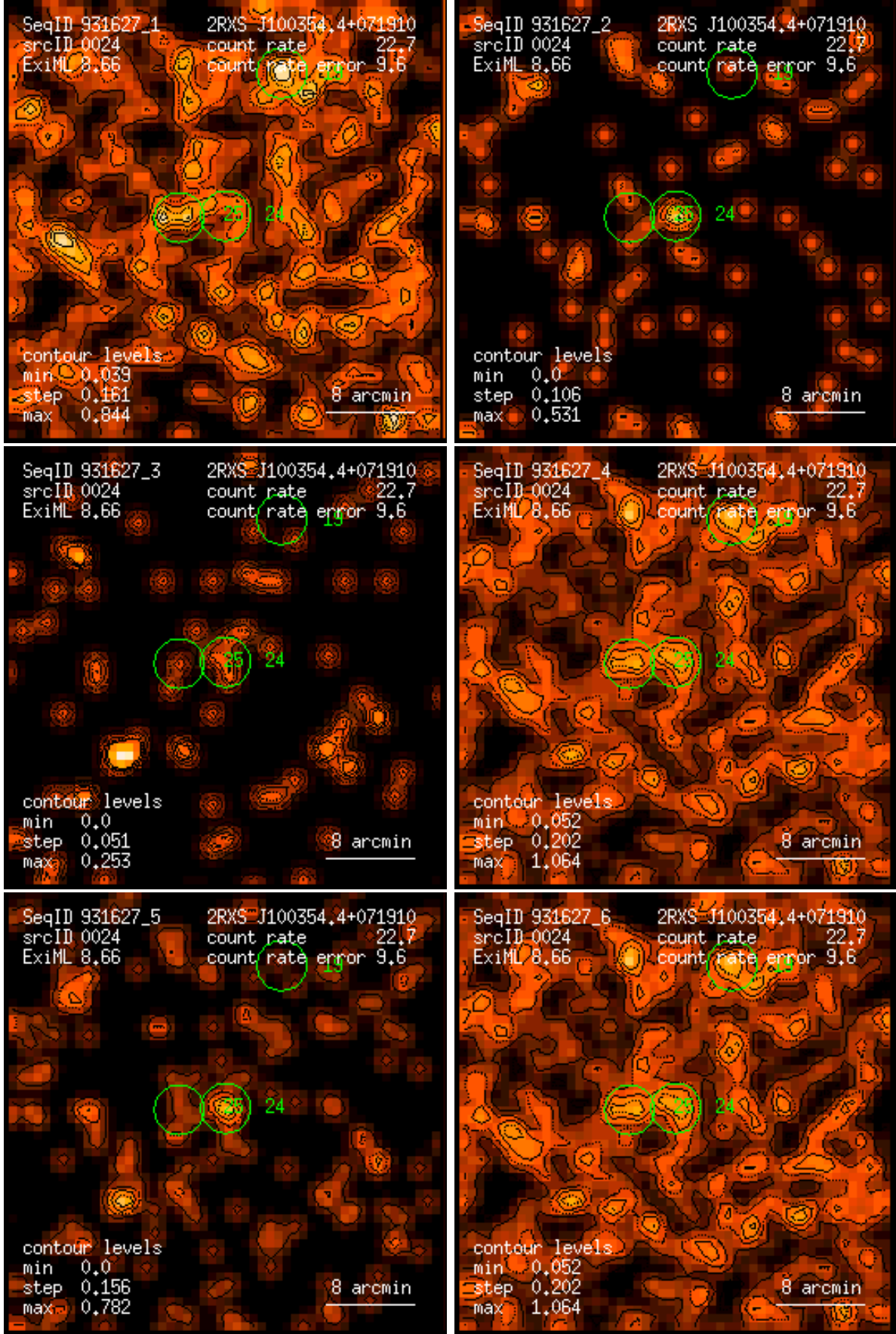
Figure 24: RASS 931627: detection 0024: band rate images, Gaussian filter: (1) PSPC channels 11 – 41, (2) 52 – 90, (3) 91 – 201, (4) 11 – 235, (5) 52 – 201, (6) 11 – 201. Broad band rates in counts/ks. Band rate contour levels in counts/ks/arcmin 2 .
