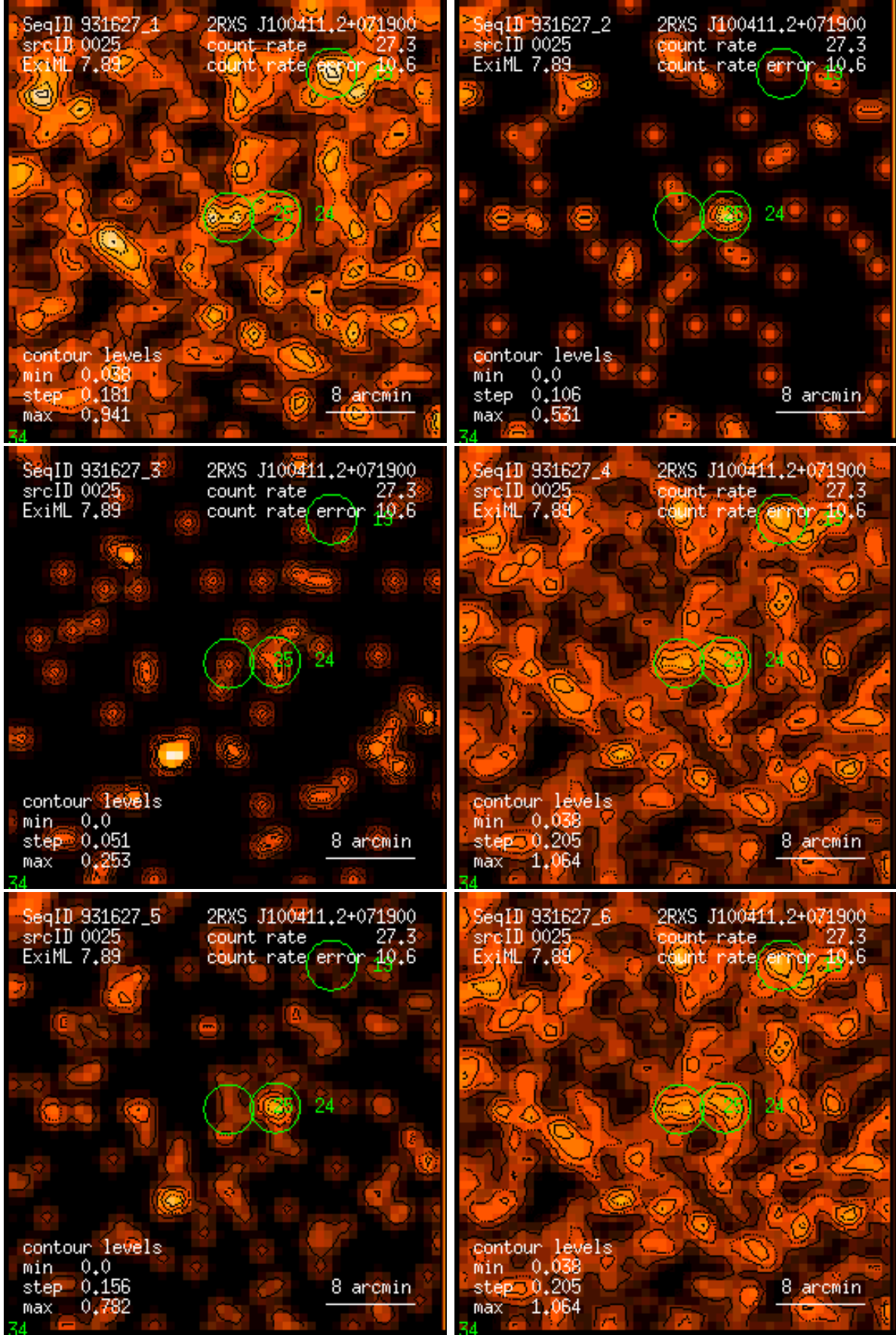
Figure 25: RASS 931627: detection 0025: band rate images, Gaussian filter: (1) PSPC channels 11 – 41, (2) 52 – 90, (3) 91 – 201, (4) 11 – 235, (5) 52 – 201, (6) 11 – 201. Broad band rates in counts/ks. Band rate contour levels in counts/ks/arcmin 2 .
