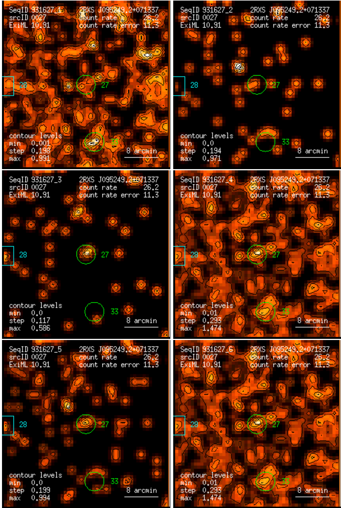
Figure 27: RASS 931627: detection 0027: band rate images, Gaussian filter: (1) PSPC channels 11 – 41, (2) 52 – 90, (3) 91 – 201, (4) 11 – 235, (5) 52 – 201, (6) 11 – 201. Broad band rates in counts/ks. Band rate contour levels in counts/ks/arcmin 2 .
